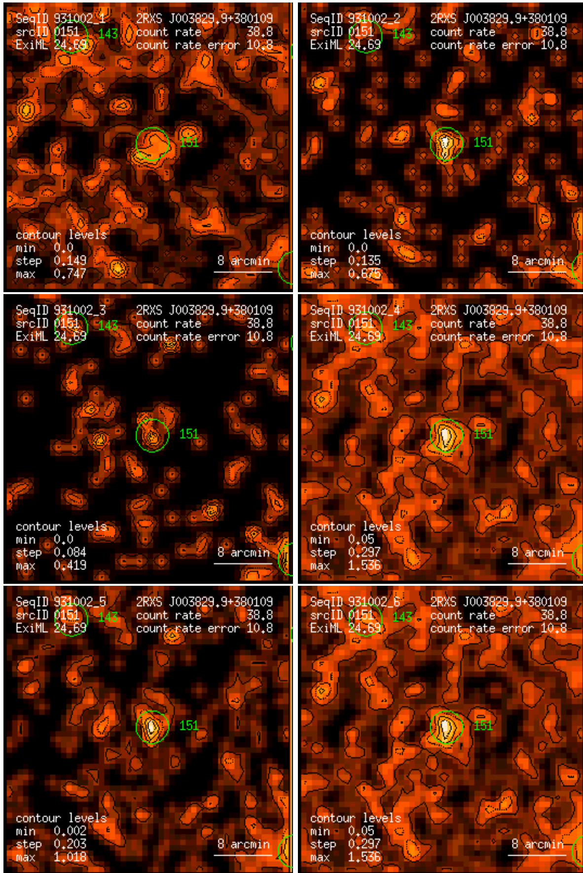
Figure 151: RASS 931002: detection 0151: band rate images, Gaussian filter: (1) PSPC channels 11 – 41, (2) 52 – 90, (3) 91 – 201, (4) 11 – 235, (5) 52 – 201, (6) 11 – 201. Broad band rates in counts/ks. Band rate contour levels in counts/ks/arcmin 2 .
