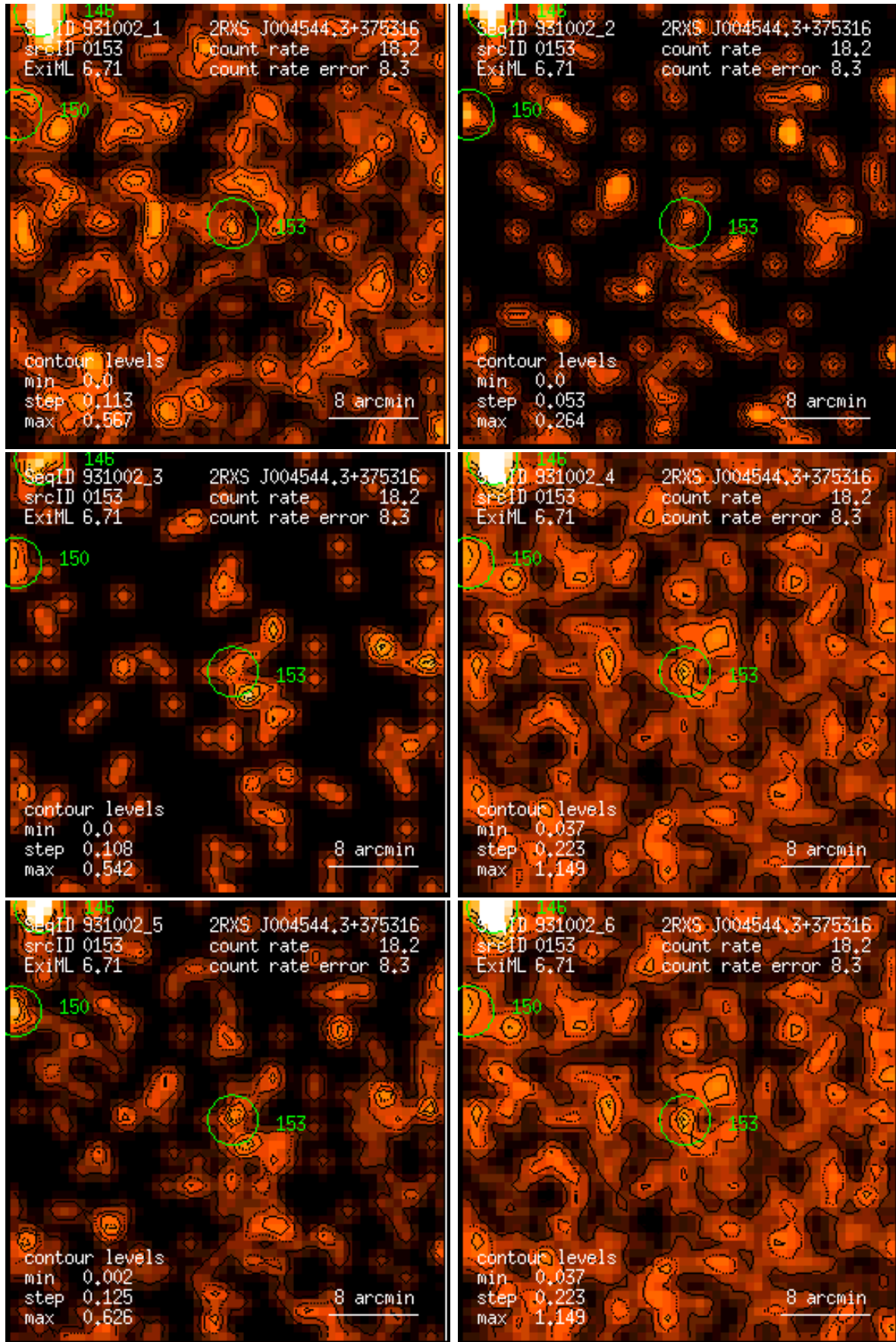
Figure 153: RASS 931002: detection 0153: band rate images, Gaussian filter: (1) PSPC channels 11 – 41, (2) 52 – 90, (3) 91 – 201, (4) 11 – 235, (5) 52 – 201, (6) 11 – 201. Broad band rates in counts/ks. Band rate contour levels in counts/ks/arcmin 2 .
