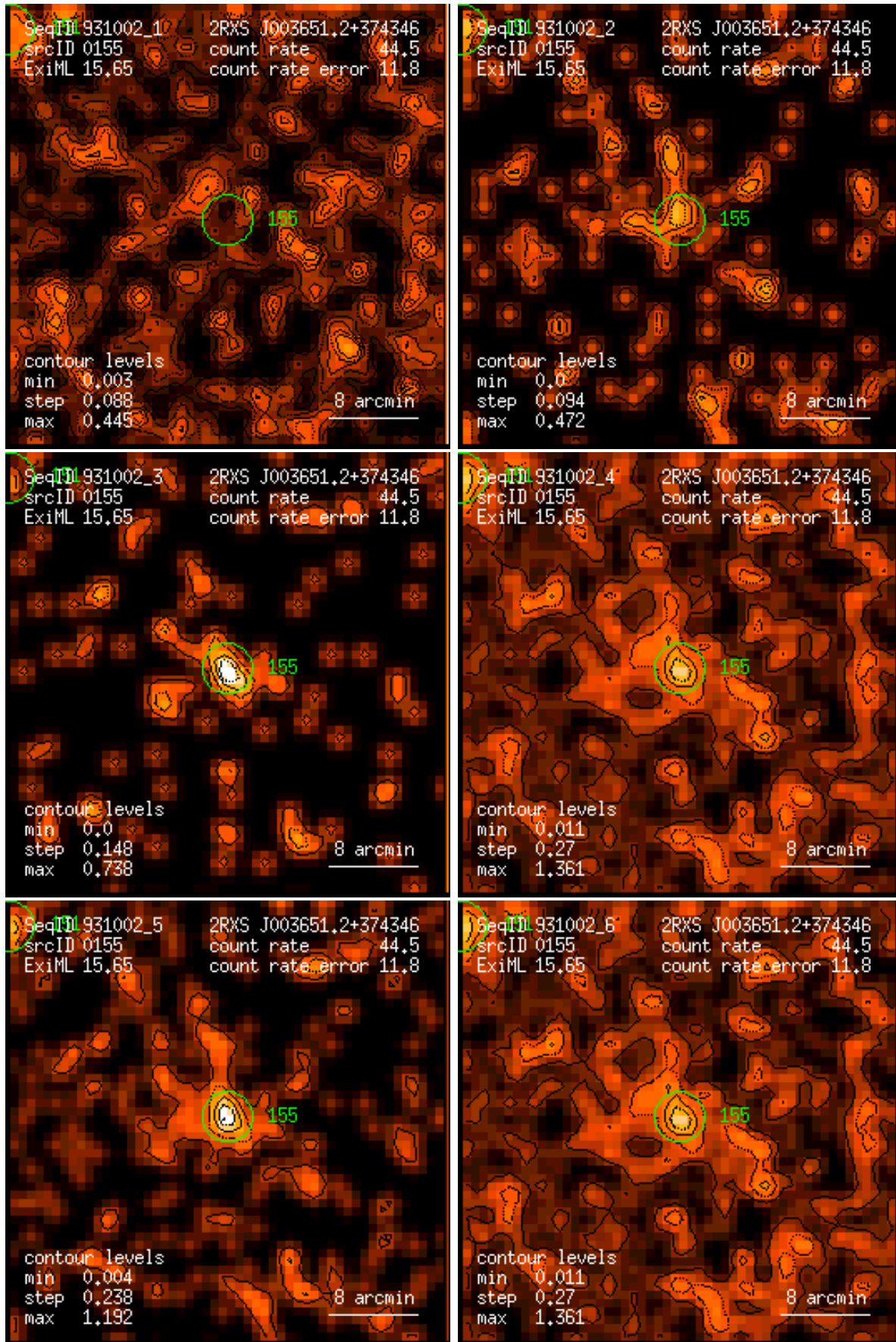
Figure 155: RASS 931002: detection 0155: band rate images, Gaussian filter: (1) PSPC channels 11 – 41, (2) 52 – 90, (3) 91 – 201, (4) 11 – 235, (5) 52 – 201, (6) 11 – 201. Broad band rates in counts/ks. Band rate contour levels in counts/ks/arcmin 2 .
