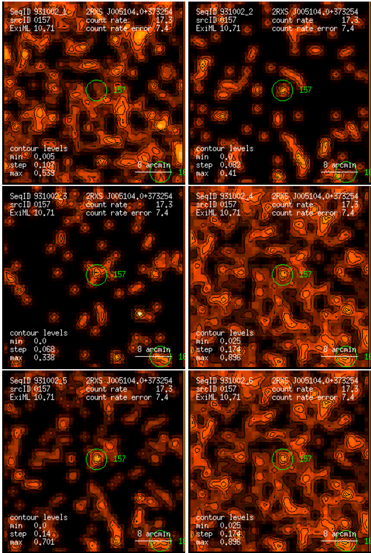
Figure 157: RASS 931002: detection 0157: band rate images, Gaussian filter: (1) PSPC channels 11 – 41, (2) 52 – 90, (3) 91 – 201, (4) 11 – 235, (5) 52 – 201, (6) 11 – 201. Broad band rates in counts/ks. Band rate contour levels in counts/ks/arcmin 2 .
