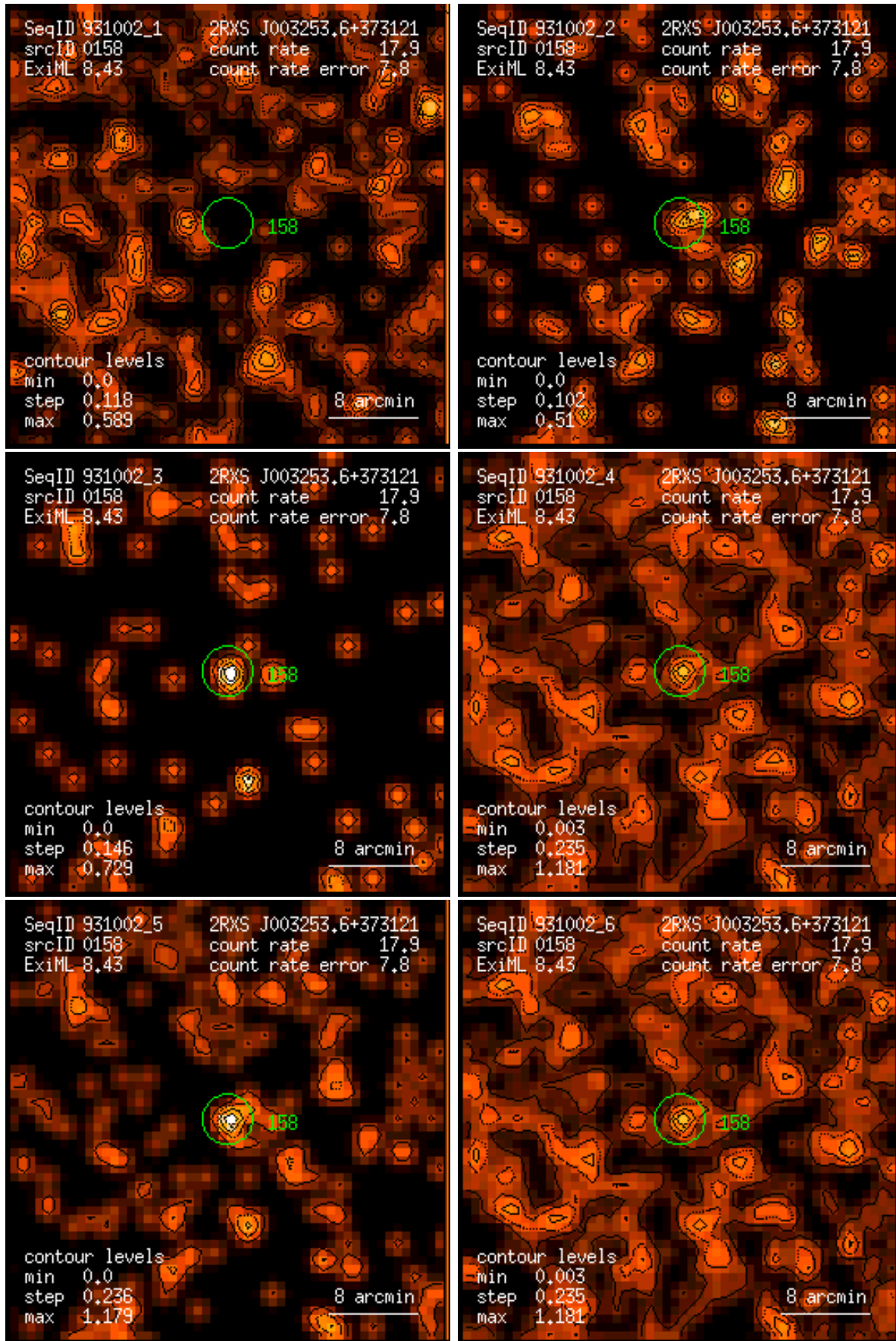
Figure 158: RASS 931002: detection 0158: band rate images, Gaussian filter: (1) PSPC channels 11 – 41, (2) 52 – 90, (3) 91 – 201, (4) 11 – 235, (5) 52 – 201, (6) 11 – 201. Broad band rates in counts/ks. Band rate contour levels in counts/ks/arcmin 2 .
