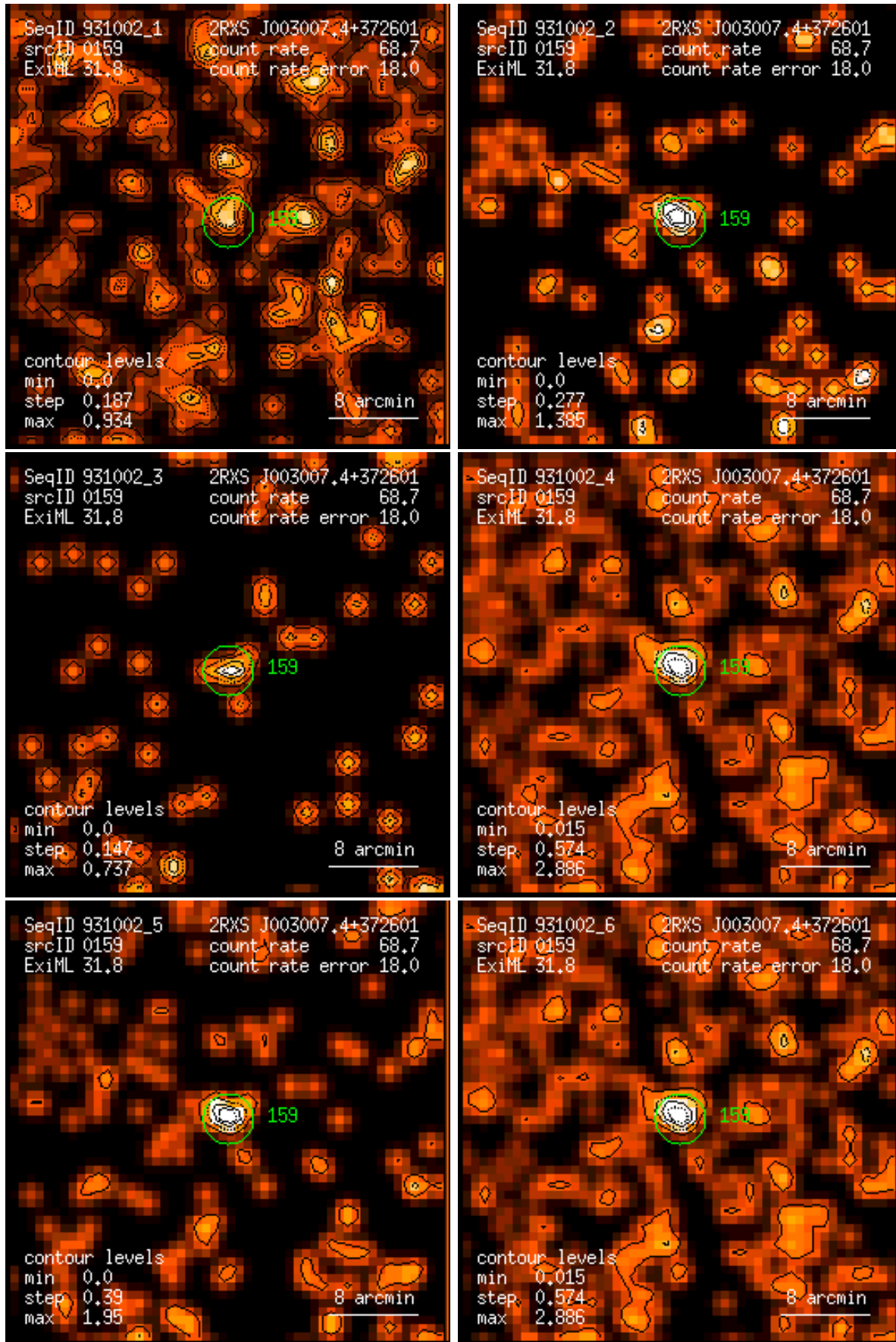
Figure 159: RASS 931002: detection 0159: band rate images, Gaussian filter: (1) PSPC channels 11 – 41, (2) 52 – 90, (3) 91 – 201, (4) 11 – 235, (5) 52 – 201, (6) 11 – 201. Broad band rates in counts/ks. Band rate contour levels in counts/ks/arcmin 2 .
