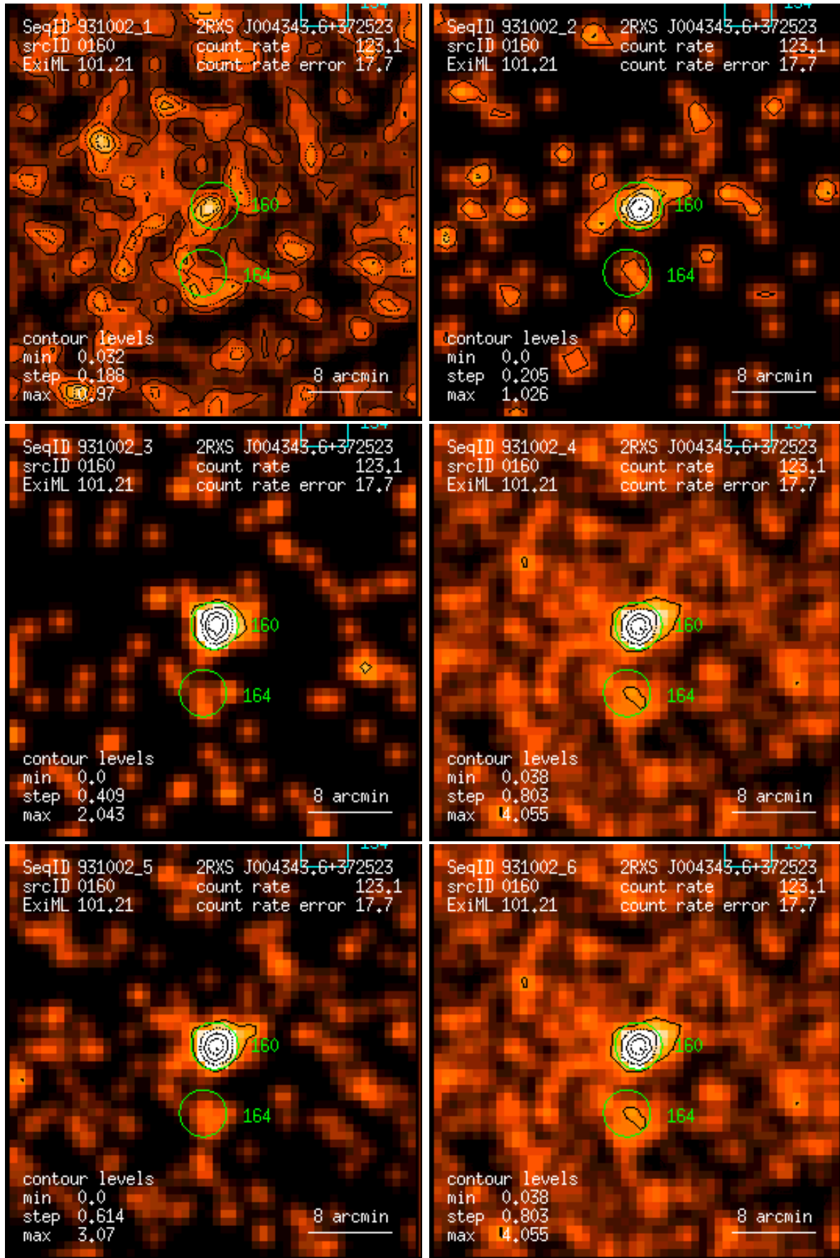
Figure 160: RASS 931002: detection 0160: band rate images, Gaussian filter: (1) PSPC channels 11 – 41, (2) 52 – 90, (3) 91 – 201, (4) 11 – 235, (5) 52 – 201, (6) 11 – 201. Broad band rates in counts/ks. Band rate contour levels in counts/ks/arcmin 2 .
