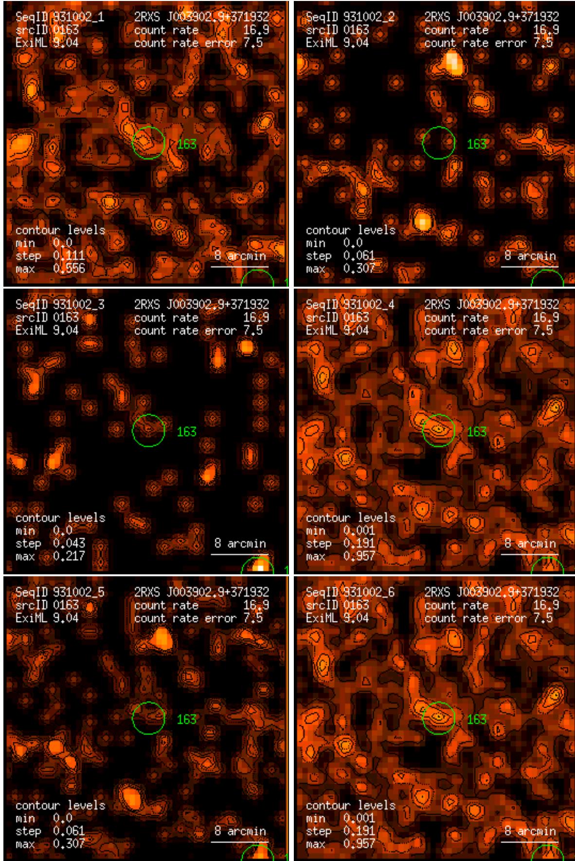
Figure 163: RASS 931002: detection 0163: band rate images, Gaussian filter: (1) PSPC channels 11 – 41, (2) 52 – 90, (3) 91 – 201, (4) 11 – 235, (5) 52 – 201, (6) 11 – 201. Broad band rates in counts/ks. Band rate contour levels in counts/ks/arcmin 2 .
