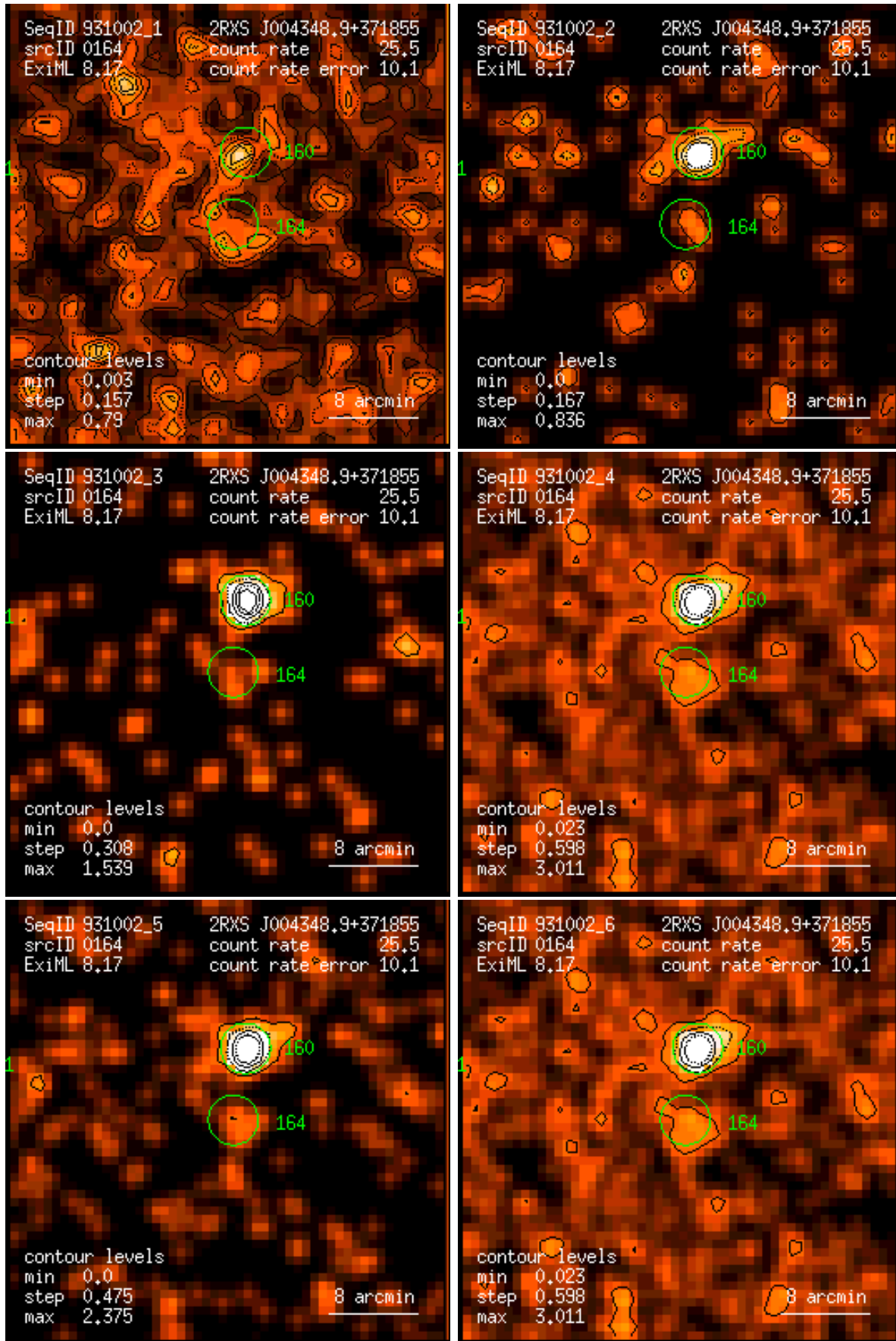
Figure 164: RASS 931002: detection 0164: band rate images, Gaussian filter: (1) PSPC channels 11 – 41, (2) 52 – 90, (3) 91 – 201, (4) 11 – 235, (5) 52 – 201, (6) 11 – 201. Broad band rates in counts/ks. Band rate contour levels in counts/ks/arcmin 2 .
