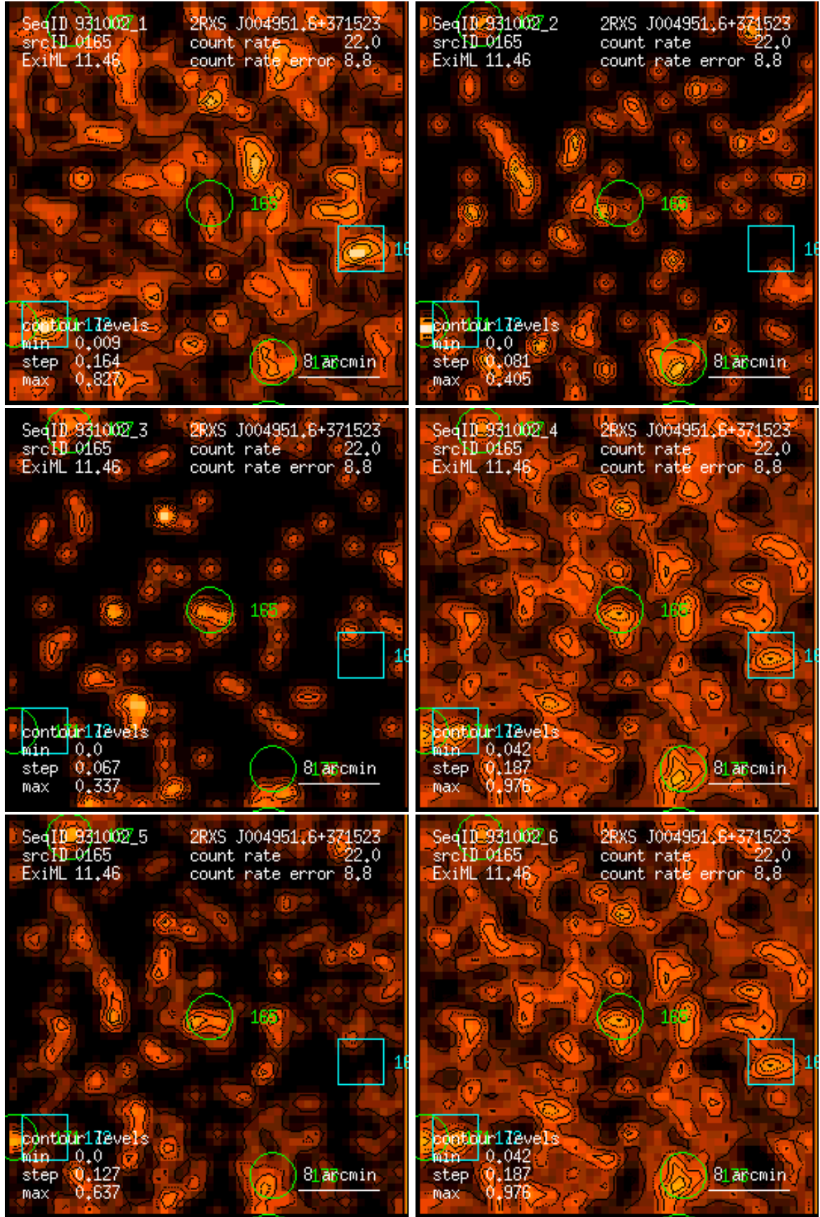
Figure 165: RASS 931002: detection 0165: band rate images, Gaussian filter: (1) PSPC channels 11 – 41, (2) 52 – 90, (3) 91 – 201, (4) 11 – 235, (5) 52 – 201, (6) 11 – 201. Broad band rates in counts/ks. Band rate contour levels in counts/ks/arcmin 2 .
