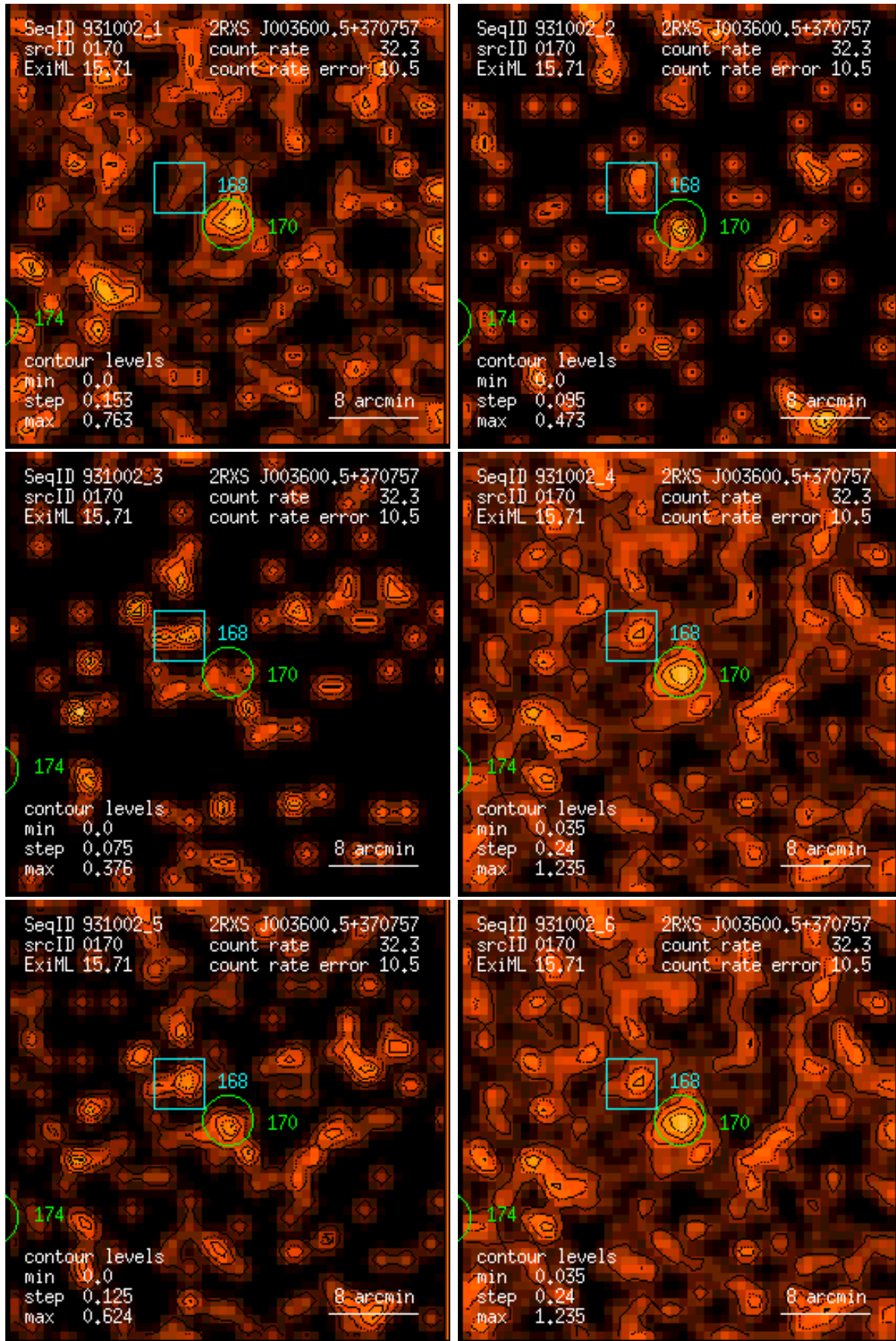
Figure 170: RASS 931002: detection 0170: band rate images, Gaussian filter: (1) PSPC channels 11 – 41, (2) 52 – 90, (3) 91 – 201, (4) 11 – 235, (5) 52 – 201, (6) 11 – 201. Broad band rates in counts/ks. Band rate contour levels in counts/ks/arcmin 2 .
