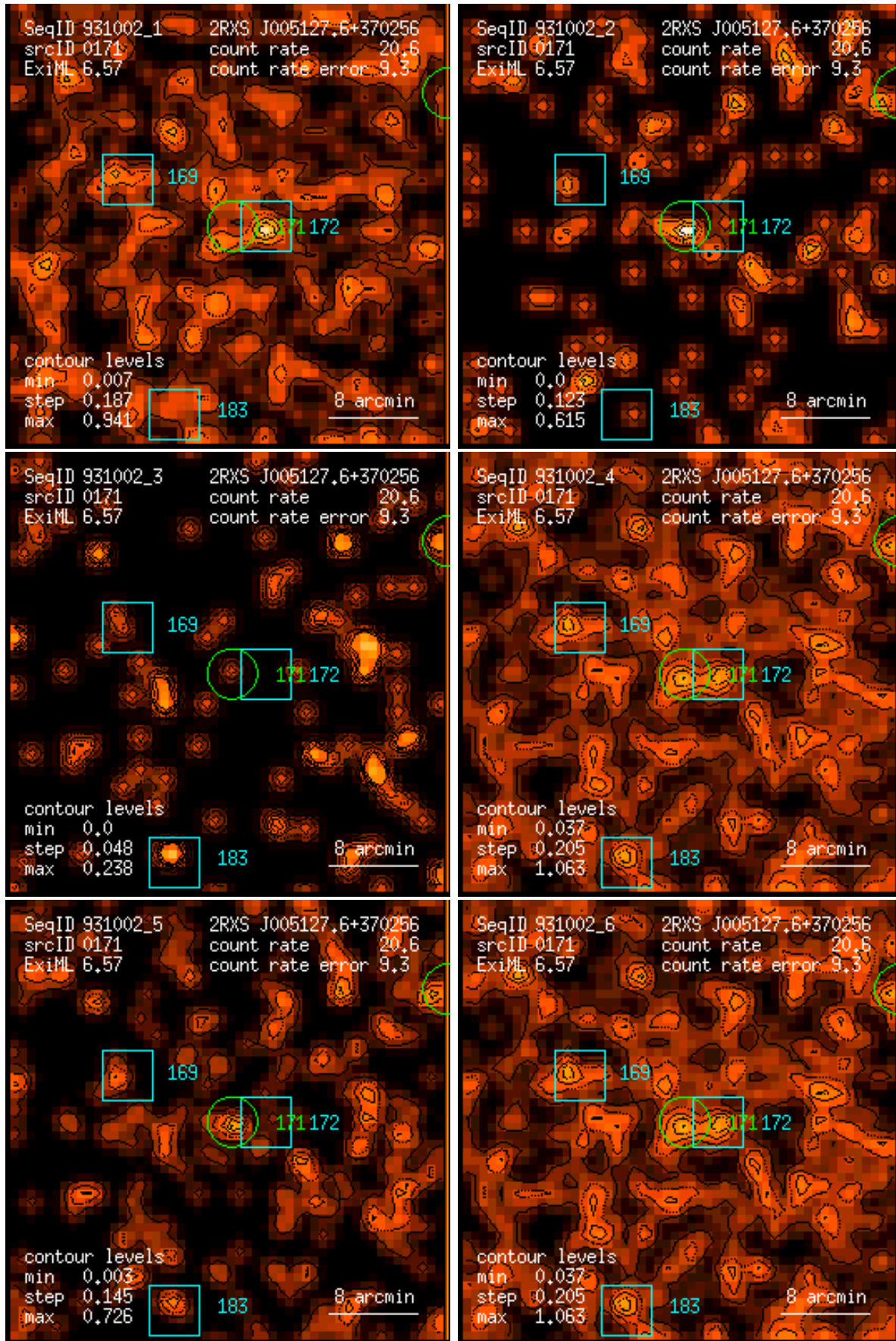
Figure 171: RASS 931002: detection 0171: band rate images, Gaussian filter: (1) PSPC channels 11 – 41, (2) 52 – 90, (3) 91 – 201, (4) 11 – 235, (5) 52 – 201, (6) 11 – 201. Broad band rates in counts/ks. Band rate contour levels in counts/ks/arcmin 2 .
