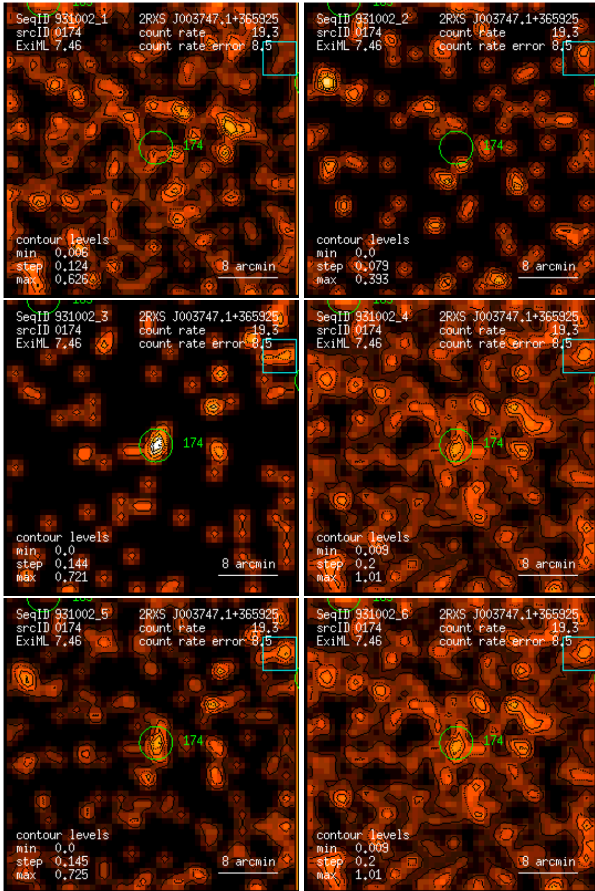
Figure 174: RASS 931002: detection 0174: band rate images, Gaussian filter: (1) PSPC channels 11 – 41, (2) 52 – 90, (3) 91 – 201, (4) 11 – 235, (5) 52 – 201, (6) 11 – 201. Broad band rates in counts/ks. Band rate contour levels in counts/ks/arcmin 2 .
