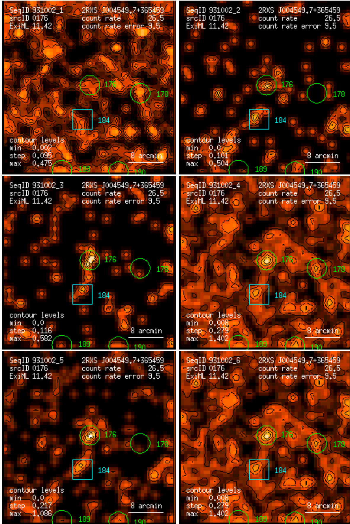
Figure 176: RASS 931002: detection 0176: band rate images, Gaussian filter: (1) PSPC channels 11 – 41, (2) 52 – 90, (3) 91 – 201, (4) 11 – 235, (5) 52 – 201, (6) 11 – 201. Broad band rates in counts/ks. Band rate contour levels in counts/ks/arcmin 2 .
