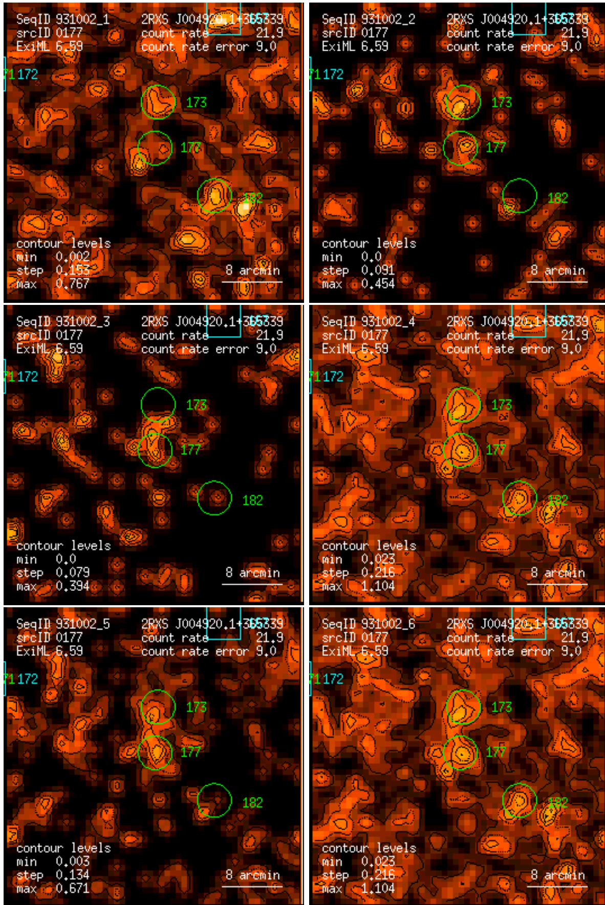
Figure 177: RASS 931002: detection 0177: band rate images, Gaussian filter: (1) PSPC channels 11 – 41, (2) 52 – 90, (3) 91 – 201, (4) 11 – 235, (5) 52 – 201, (6) 11 – 201. Broad band rates in counts/ks. Band rate contour levels in counts/ks/arcmin 2 .
