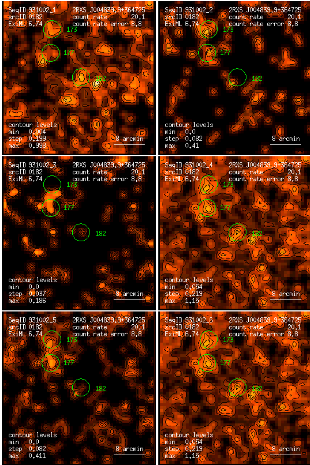
Figure 182: RASS 931002: detection 0182: band rate images, Gaussian filter: (1) PSPC channels 11 – 41, (2) 52 – 90, (3) 91 – 201, (4) 11 – 235, (5) 52 – 201, (6) 11 – 201. Broad band rates in counts/ks. Band rate contour levels in counts/ks/arcmin 2 .
