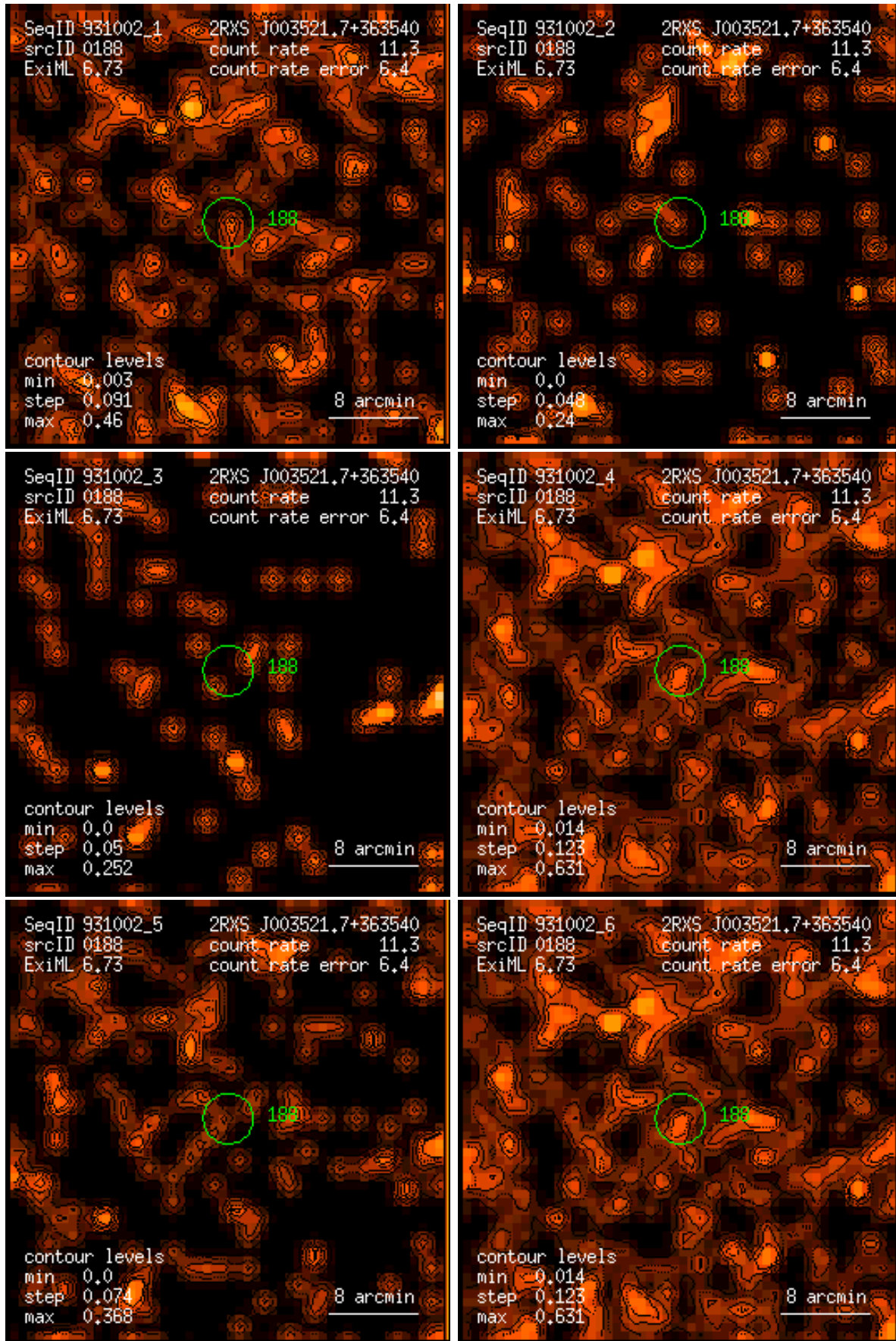
Figure 188: RASS 931002: detection 0188: band rate images, Gaussian filter: (1) PSPC channels 11 – 41, (2) 52 – 90, (3) 91 – 201, (4) 11 – 235, (5) 52 – 201, (6) 11 – 201. Broad band rates in counts/ks. Band rate contour levels in counts/ks/arcmin 2 .
