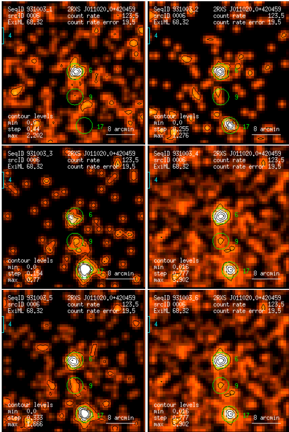
Figure 6: RASS 931003: detection 0006: band rate images, Gaussian filter: (1) PSPC channels 11 – 41, (2) 52 – 90, (3) 91 – 201, (4) 11 – 235, (5) 52 – 201, (6) 11 – 201. Broad band rates in counts/ks. Band rate contour levels in counts/ks/arcmin 2 .
