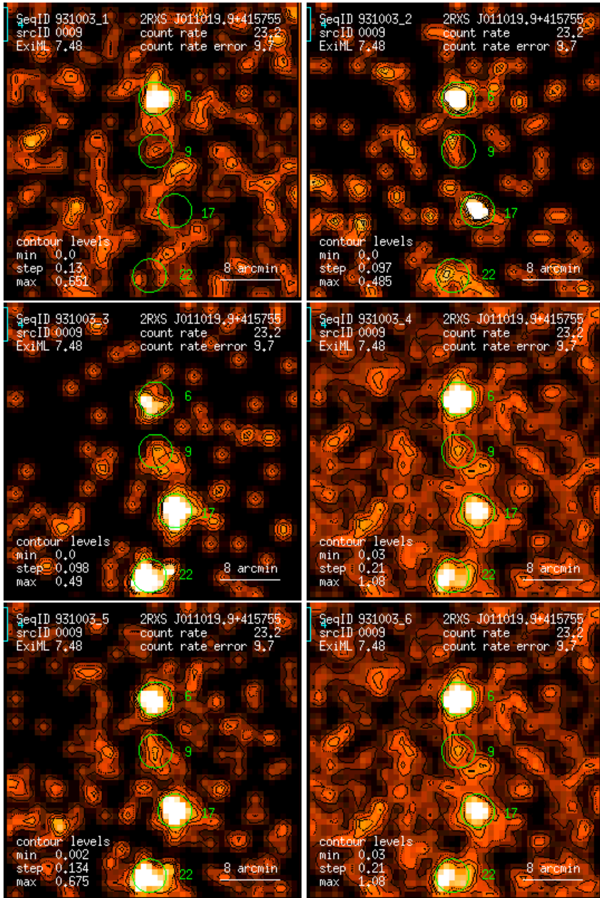
Figure 9: RASS 931003: detection 0009: band rate images, Gaussian filter: (1) PSPC channels 11 – 41, (2) 52 – 90, (3) 91 – 201, (4) 11 – 235, (5) 52 – 201, (6) 11 – 201. Broad band rates in counts/ks. Band rate contour levels in counts/ks/arcmin 2 .
