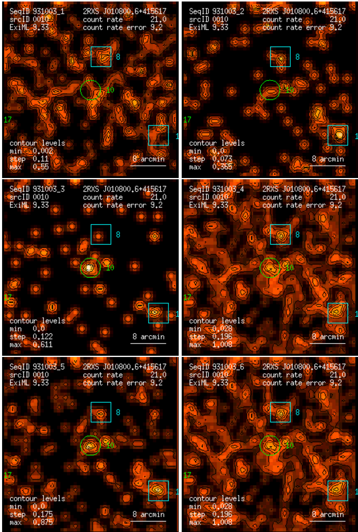
Figure 10: RASS 931003: detection 0010: band rate images, Gaussian filter: (1) PSPC channels 11 – 41, (2) 52 – 90, (3) 91 – 201, (4) 11 – 235, (5) 52 – 201, (6) 11 – 201. Broad band rates in counts/ks. Band rate contour levels in counts/ks/arcmin 2 .
