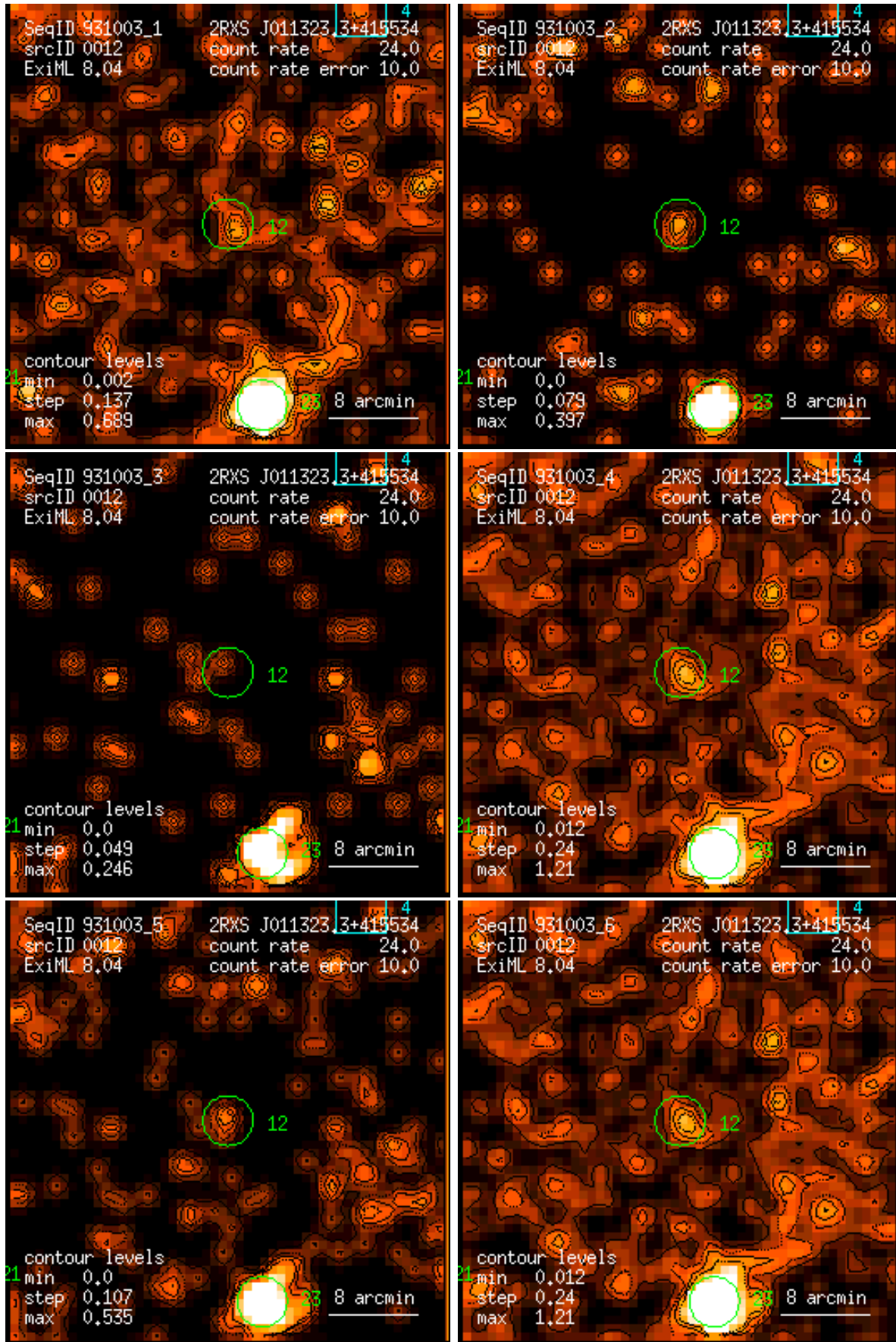
Figure 12: RASS 931003: detection 0012: band rate images, Gaussian filter: (1) PSPC channels 11 – 41, (2) 52 – 90, (3) 91 – 201, (4) 11 – 235, (5) 52 – 201, (6) 11 – 201. Broad band rates in counts/ks. Band rate contour levels in counts/ks/arcmin 2 .
