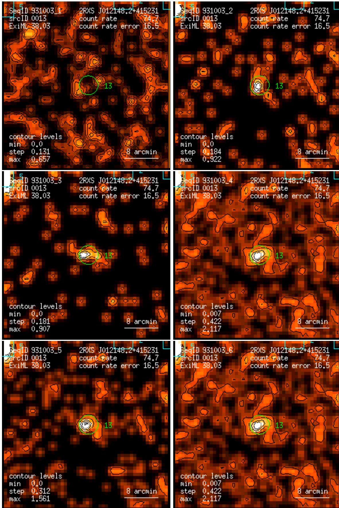
Figure 13: RASS 931003: detection 0013: band rate images, Gaussian filter: (1) PSPC channels 11 – 41, (2) 52 – 90, (3) 91 – 201, (4) 11 – 235, (5) 52 – 201, (6) 11 – 201. Broad band rates in counts/ks. Band rate contour levels in counts/ks/arcmin 2 .
