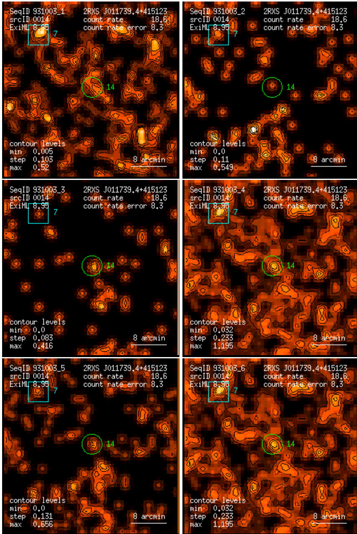
Figure 14: RASS 931003: detection 0014: band rate images, Gaussian filter: (1) PSPC channels 11 – 41, (2) 52 – 90, (3) 91 – 201, (4) 11 – 235, (5) 52 – 201, (6) 11 – 201. Broad band rates in counts/ks. Band rate contour levels in counts/ks/arcmin 2 .
