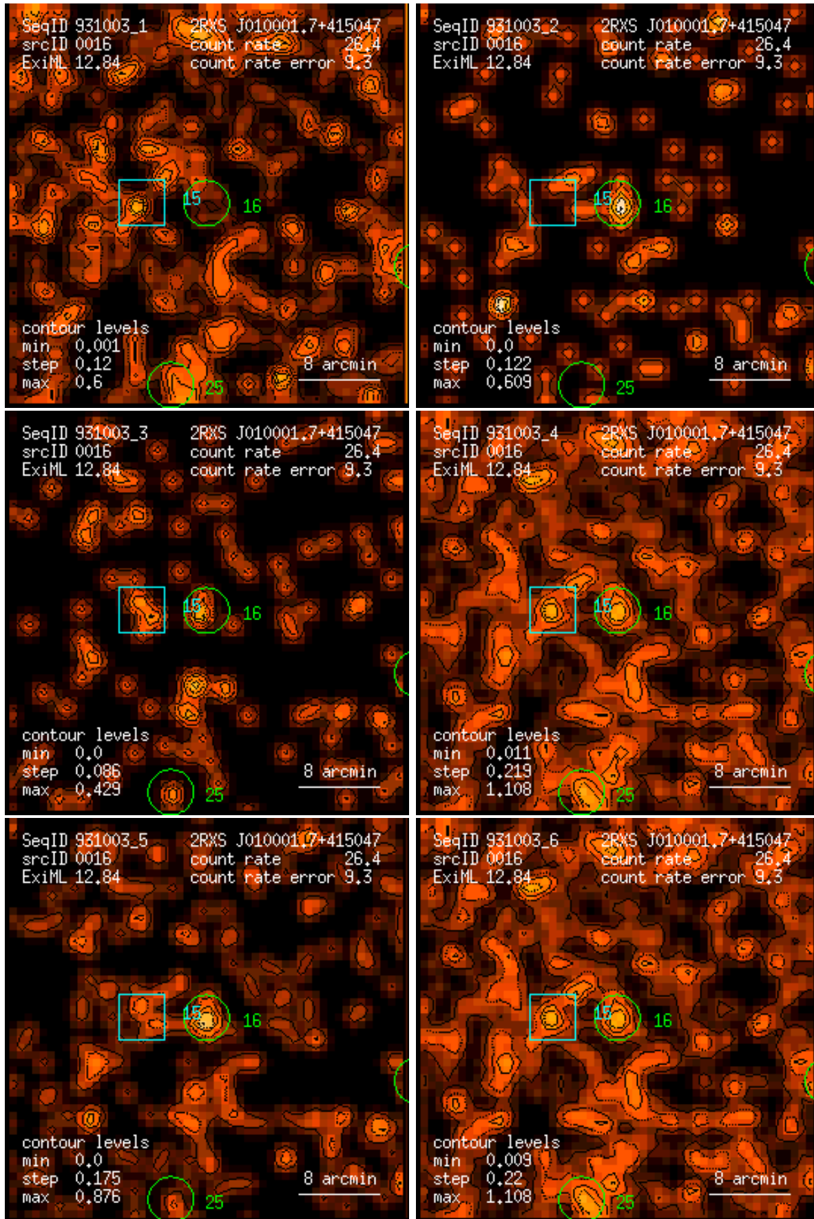
Figure 16: RASS 931003: detection 0016: band rate images, Gaussian filter: (1) PSPC channels 11 – 41, (2) 52 – 90, (3) 91 – 201, (4) 11 – 235, (5) 52 – 201, (6) 11 – 201. Broad band rates in counts/ks. Band rate contour levels in counts/ks/arcmin 2 .
