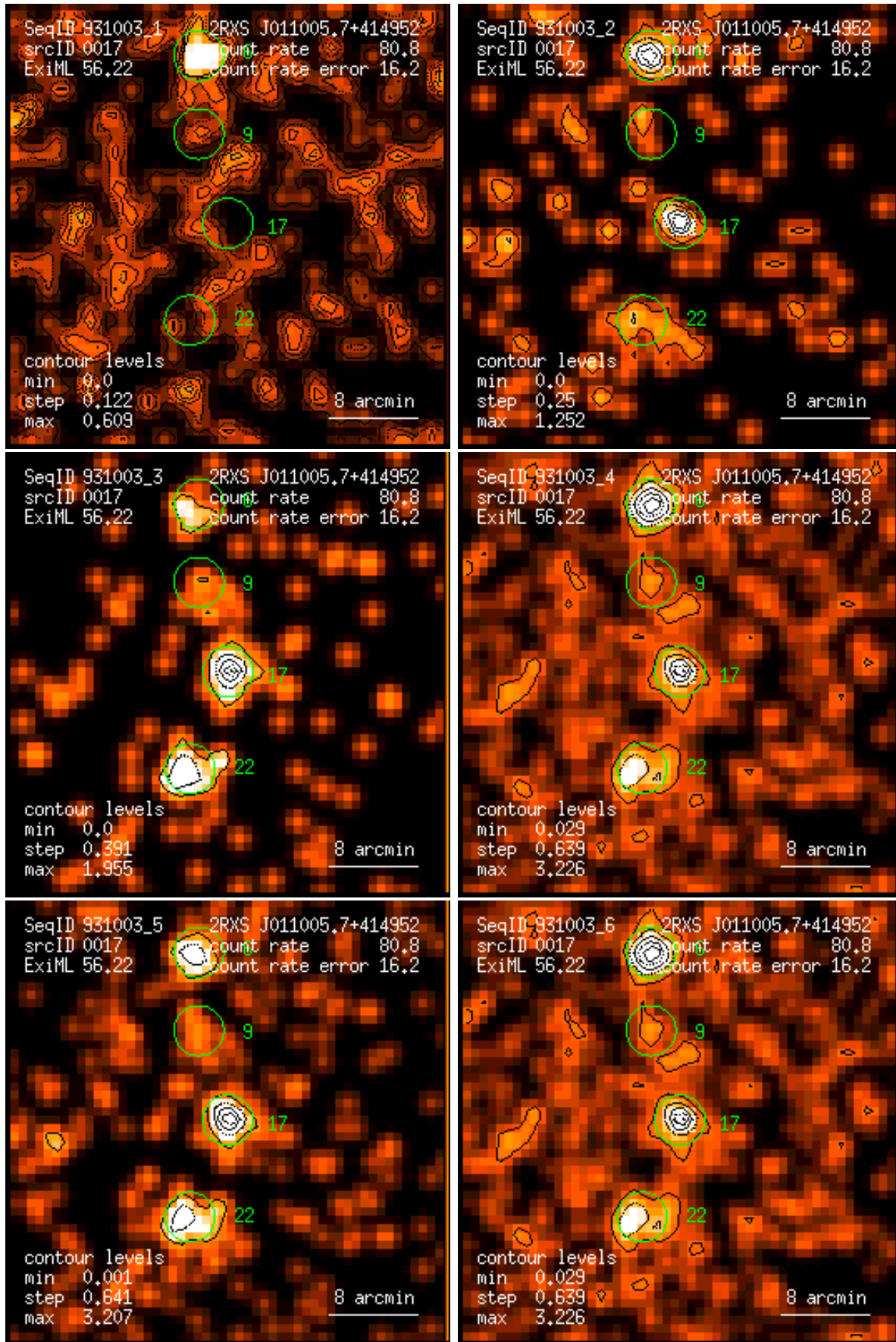
Figure 17: RASS 931003: detection 0017: band rate images, Gaussian filter: (1) PSPC channels 11 – 41, (2) 52 – 90, (3) 91 – 201, (4) 11 – 235, (5) 52 – 201, (6) 11 – 201. Broad band rates in counts/ks. Band rate contour levels in counts/ks/arcmin 2 .
