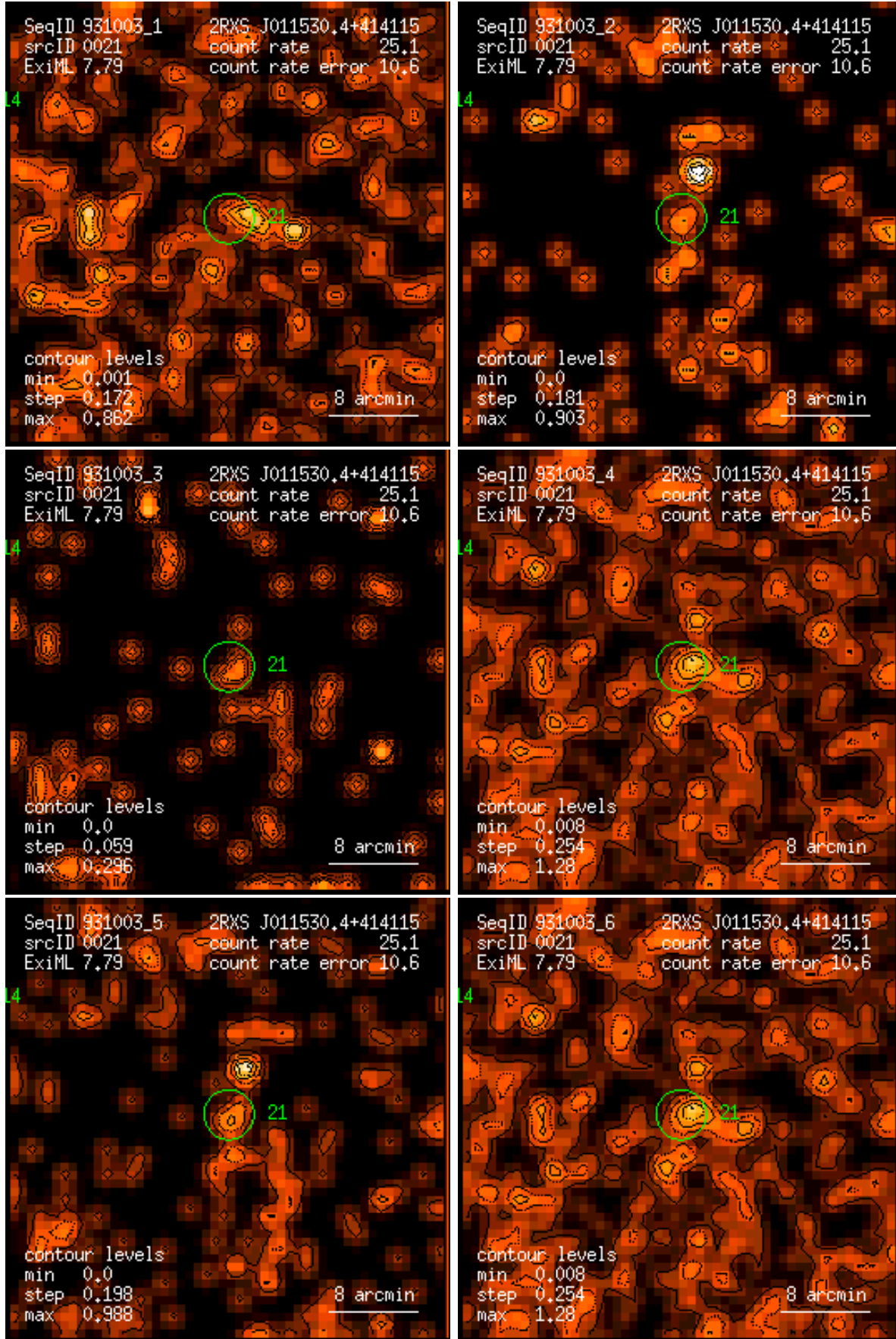
Figure 21: RASS 931003: detection 0021: band rate images, Gaussian filter: (1) PSPC channels 11 – 41, (2) 52 – 90, (3) 91 – 201, (4) 11 – 235, (5) 52 – 201, (6) 11 – 201. Broad band rates in counts/ks. Band rate contour levels in counts/ks/arcmin 2 .
