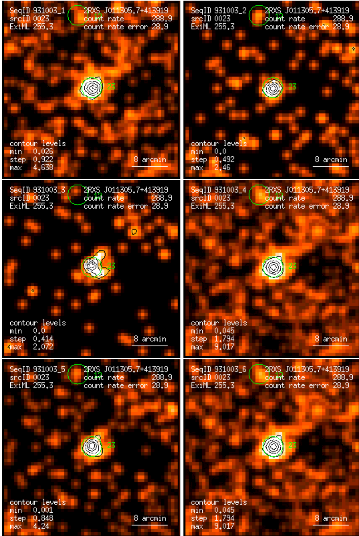
Figure 23: RASS 931003: detection 0023: band rate images, Gaussian filter: (1) PSPC channels 11 – 41, (2) 52 – 90, (3) 91 – 201, (4) 11 – 235, (5) 52 – 201, (6) 11 – 201. Broad band rates in counts/ks. Band rate contour levels in counts/ks/arcmin 2 .
