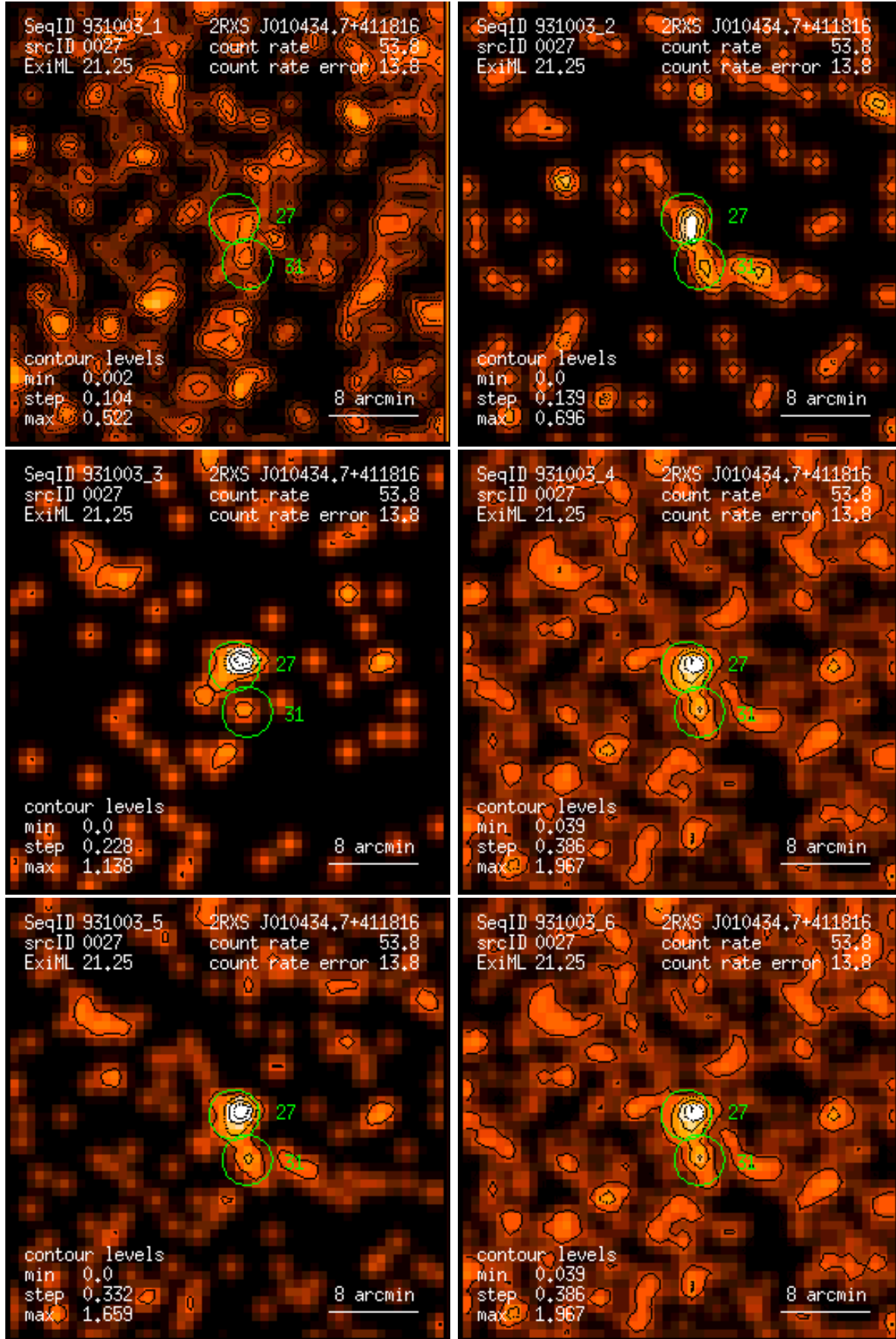
Figure 27: RASS 931003: detection 0027: band rate images, Gaussian filter: (1) PSPC channels 11 – 41, (2) 52 – 90, (3) 91 – 201, (4) 11 – 235, (5) 52 – 201, (6) 11 – 201. Broad band rates in counts/ks. Band rate contour levels in counts/ks/arcmin 2 .
