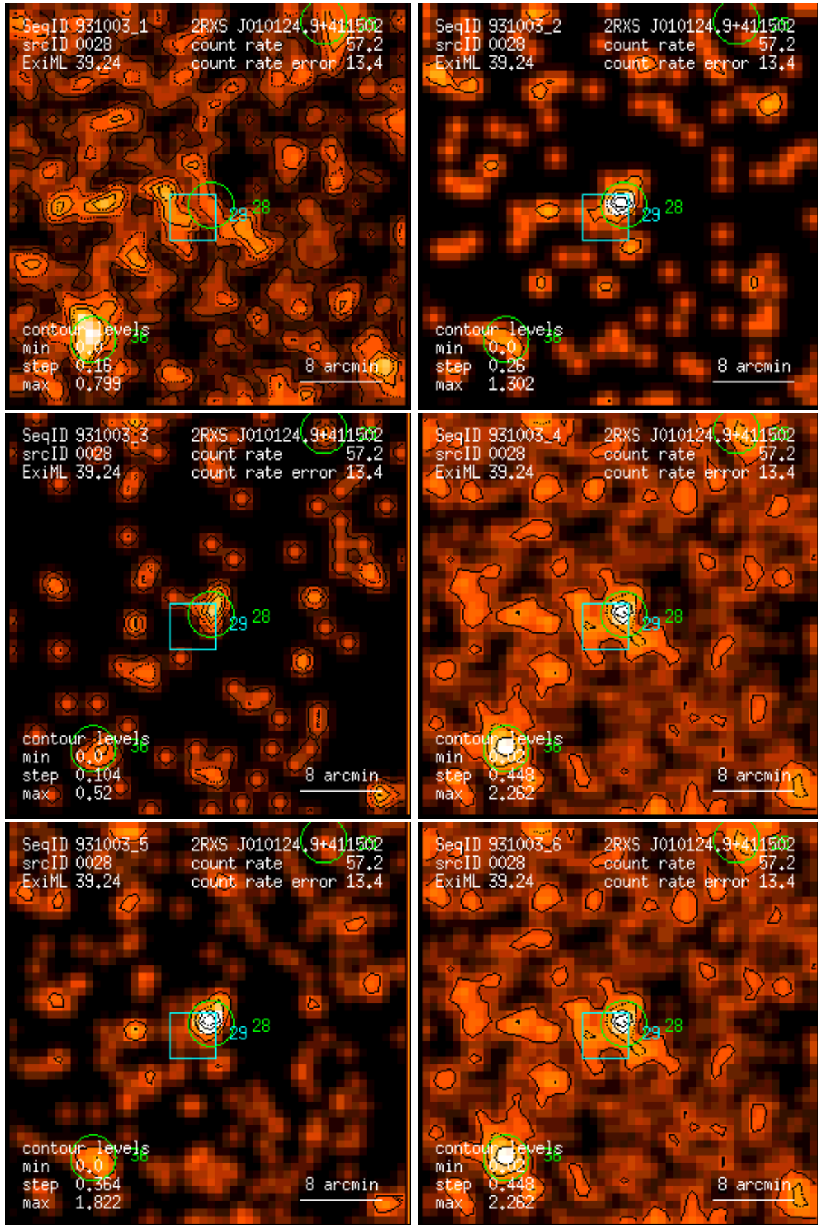
Figure 28: RASS 931003: detection 0028: band rate images, Gaussian filter: (1) PSPC channels 11 – 41, (2) 52 – 90, (3) 91 – 201, (4) 11 – 235, (5) 52 – 201, (6) 11 – 201. Broad band rates in counts/ks. Band rate contour levels in counts/ks/arcmin 2 .
