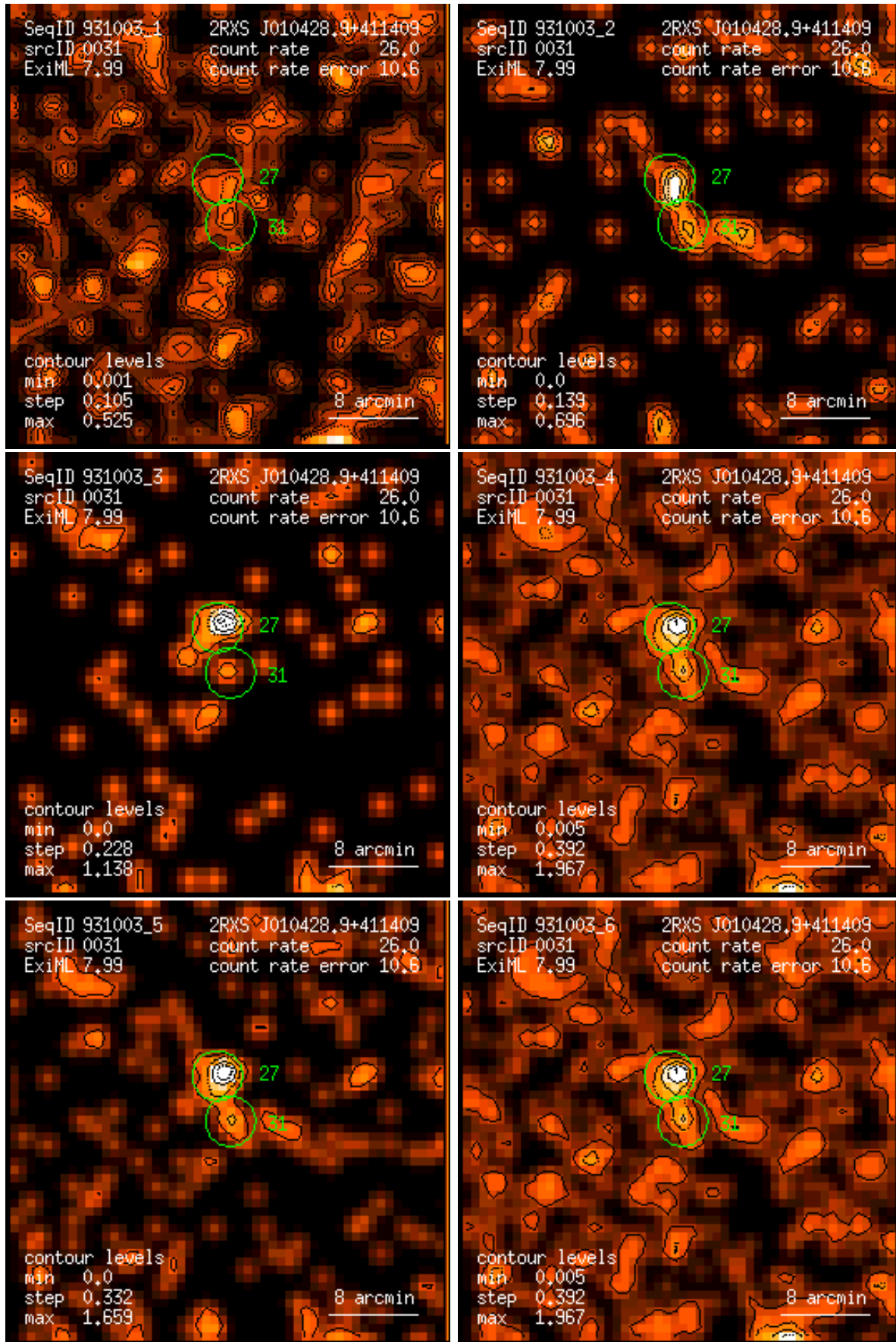
Figure 31: RASS 931003: detection 0031: band rate images, Gaussian filter: (1) PSPC channels 11 – 41, (2) 52 – 90, (3) 91 – 201, (4) 11 – 235, (5) 52 – 201, (6) 11 – 201. Broad band rates in counts/ks. Band rate contour levels in counts/ks/arcmin 2 .
