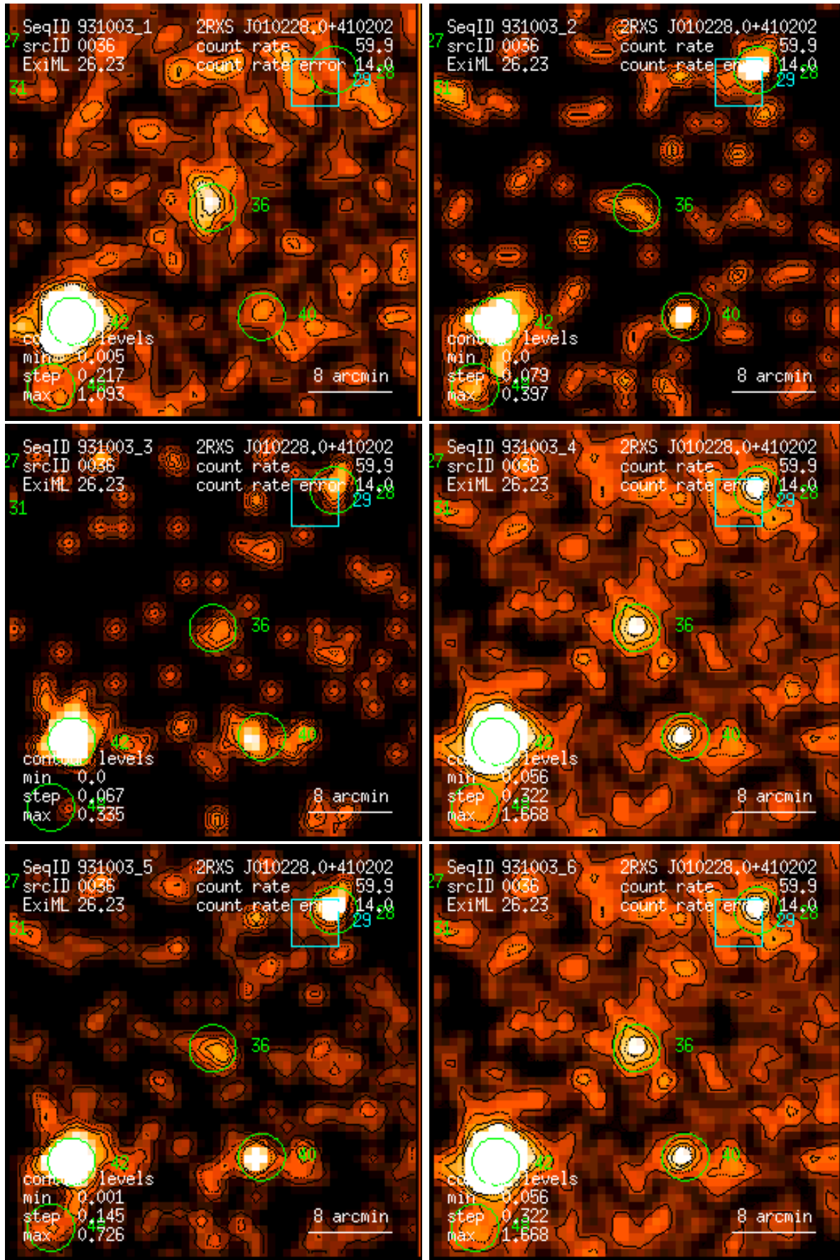
Figure 36: RASS 931003: detection 0036: band rate images, Gaussian filter: (1) PSPC channels 11 – 41, (2) 52 – 90, (3) 91 – 201, (4) 11 – 235, (5) 52 – 201, (6) 11 – 201. Broad band rates in counts/ks. Band rate contour levels in counts/ks/arcmin 2 .
