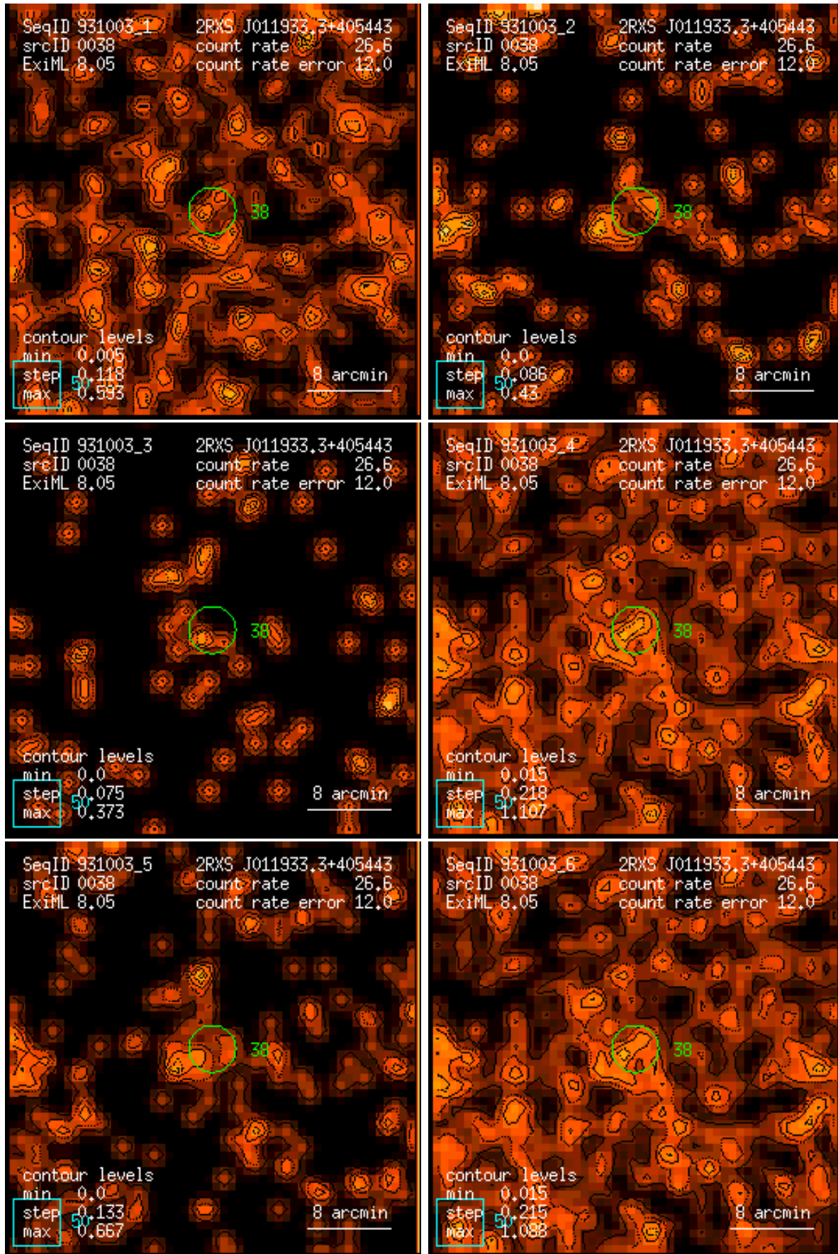
Figure 38: RASS 931003: detection 0038: band rate images, Gaussian filter: (1) PSPC channels 11 – 41, (2) 52 – 90, (3) 91 – 201, (4) 11 – 235, (5) 52 – 201, (6) 11 – 201. Broad band rates in counts/ks. Band rate contour levels in counts/ks/arcmin 2 .
