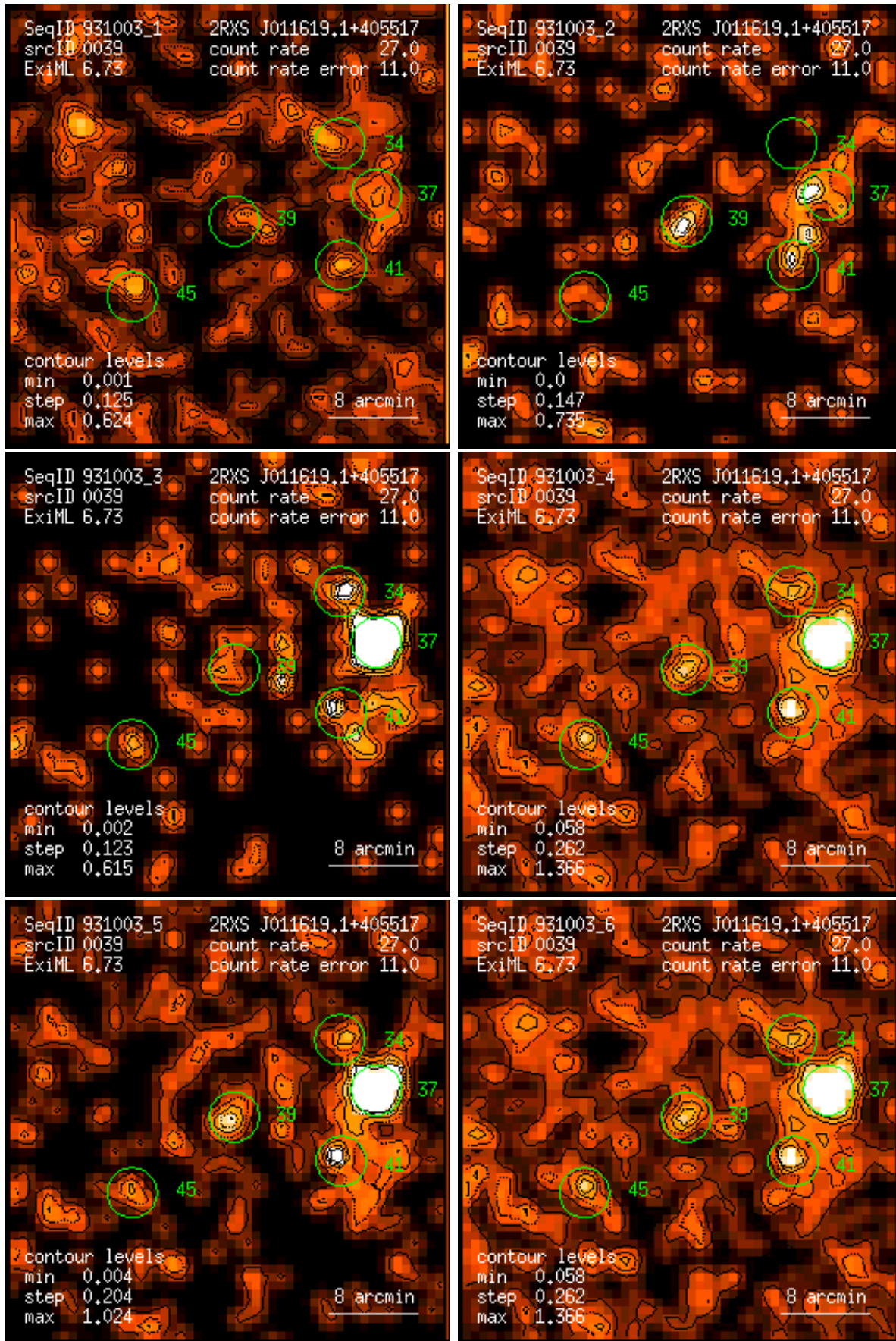
Figure 39: RASS 931003: detection 0039: band rate images, Gaussian filter: (1) PSPC channels 11 – 41, (2) 52 – 90, (3) 91 – 201, (4) 11 – 235, (5) 52 – 201, (6) 11 – 201. Broad band rates in counts/ks. Band rate contour levels in counts/ks/arcmin 2 .
