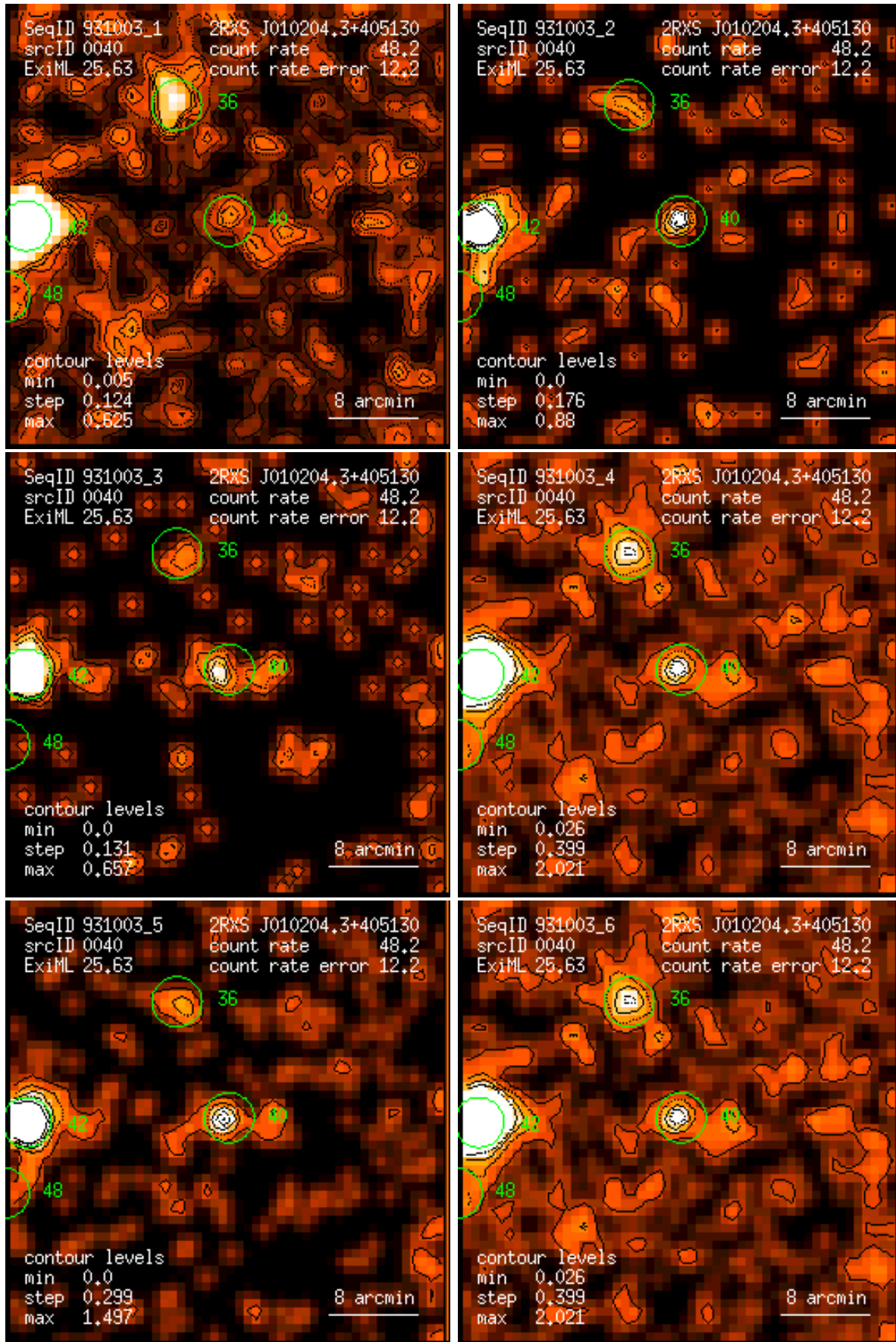
Figure 40: RASS 931003: detection 0040: band rate images, Gaussian filter: (1) PSPC channels 11 – 41, (2) 52 – 90, (3) 91 – 201, (4) 11 – 235, (5) 52 – 201, (6) 11 – 201. Broad band rates in counts/ks. Band rate contour levels in counts/ks/arcmin 2 .
