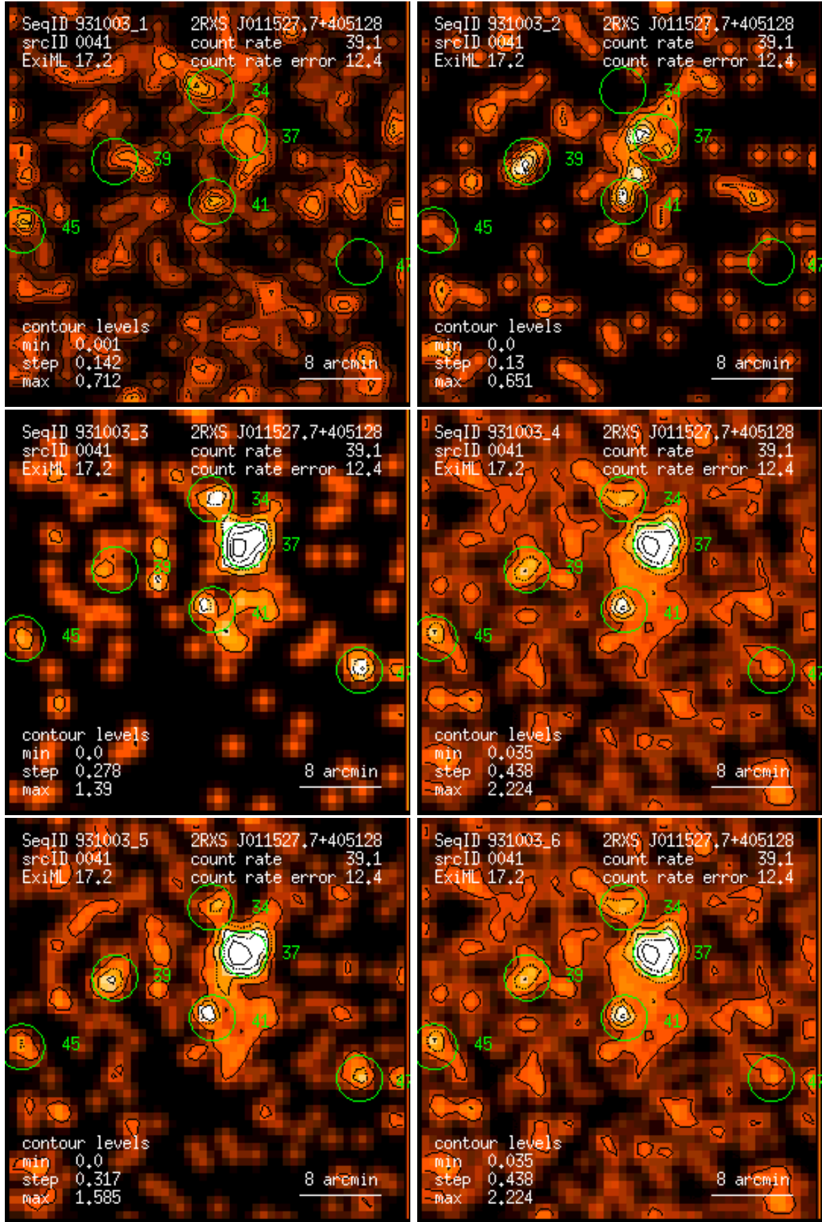
Figure 41: RASS 931003: detection 0041: band rate images, Gaussian filter: (1) PSPC channels 11 – 41, (2) 52 – 90, (3) 91 – 201, (4) 11 – 235, (5) 52 – 201, (6) 11 – 201. Broad band rates in counts/ks. Band rate contour levels in counts/ks/arcmin 2 .
