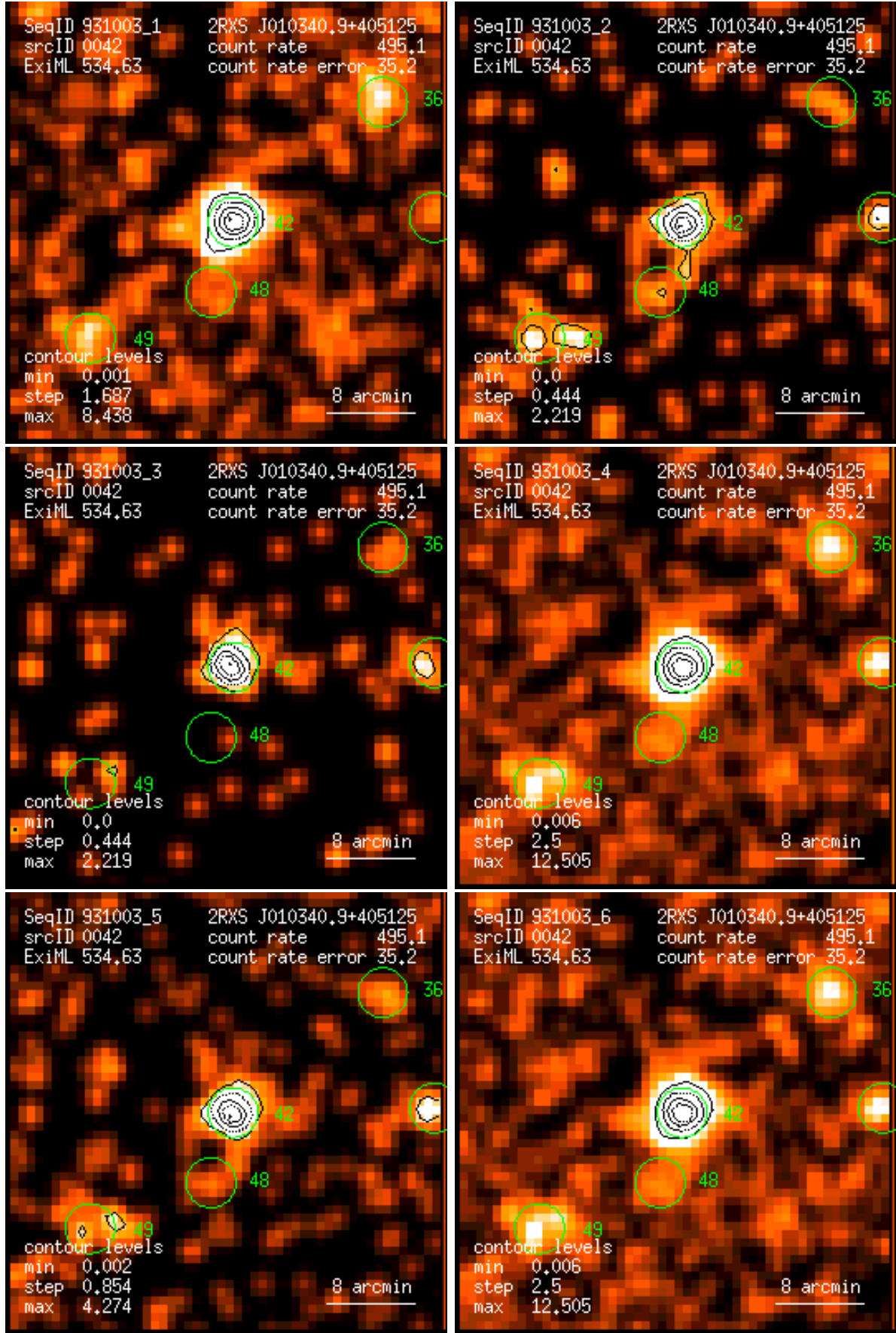
Figure 42: RASS 931003: detection 0042: band rate images, Gaussian filter: (1) PSPC channels 11 – 41, (2) 52 – 90, (3) 91 – 201, (4) 11 – 235, (5) 52 – 201, (6) 11 – 201. Broad band rates in counts/ks. Band rate contour levels in counts/ks/arcmin 2 .
