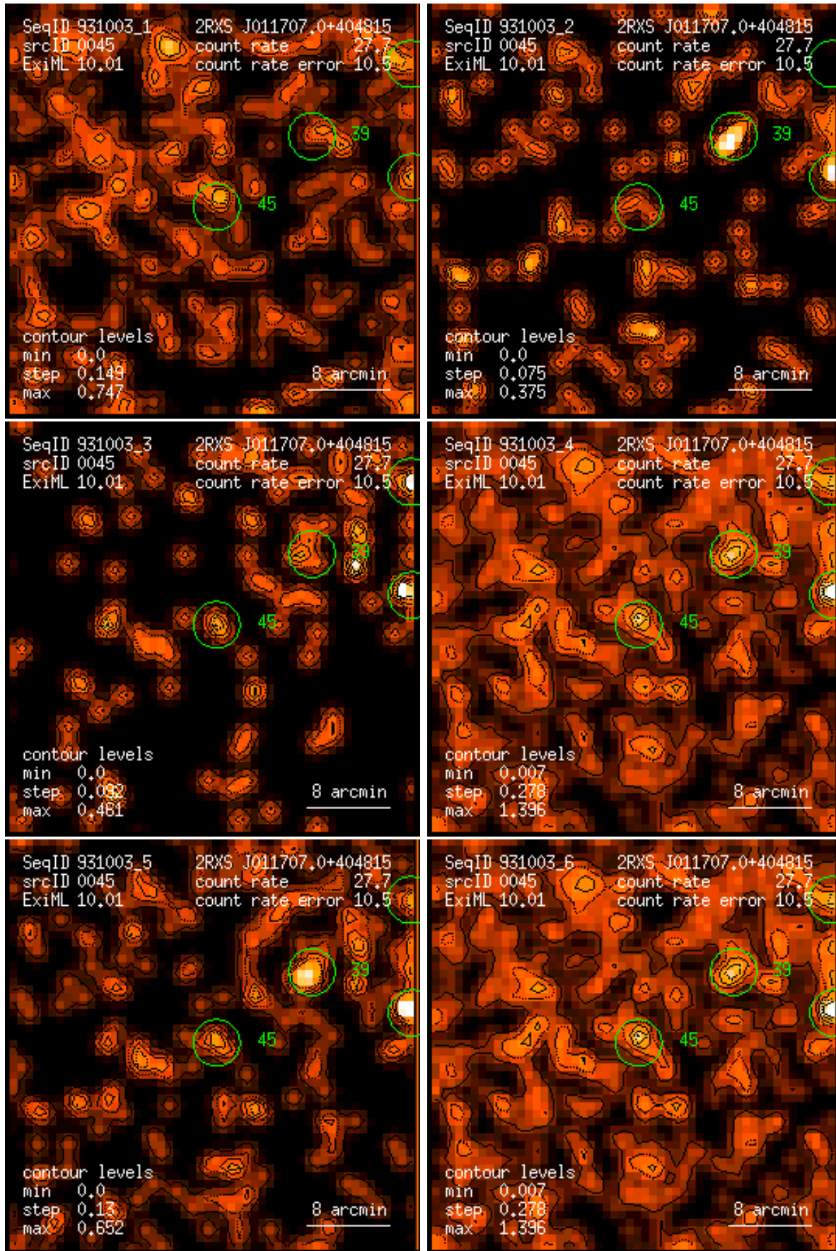
Figure 45: RASS 931003: detection 0045: band rate images, Gaussian filter: (1) PSPC channels 11 – 41, (2) 52 – 90, (3) 91 – 201, (4) 11 – 235, (5) 52 – 201, (6) 11 – 201. Broad band rates in counts/ks. Band rate contour levels in counts/ks/arcmin 2 .
