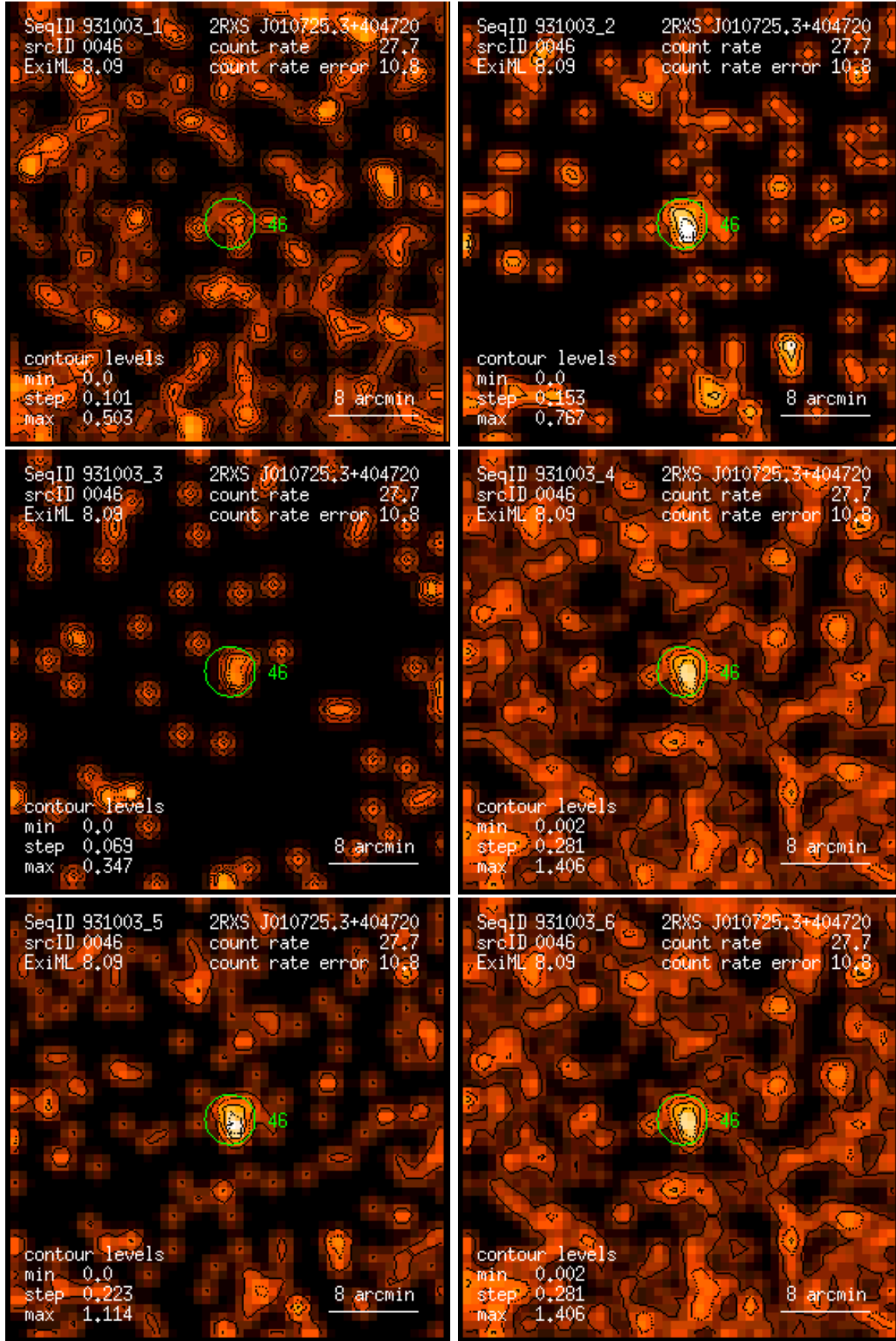
Figure 46: RASS 931003: detection 0046: band rate images, Gaussian filter: (1) PSPC channels 11 – 41, (2) 52 – 90, (3) 91 – 201, (4) 11 – 235, (5) 52 – 201, (6) 11 – 201. Broad band rates in counts/ks. Band rate contour levels in counts/ks/arcmin 2 .
