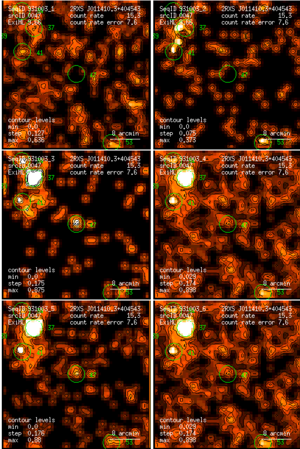
Figure 47: RASS 931003: detection 0047: band rate images, Gaussian filter: (1) PSPC channels 11 – 41, (2) 52 – 90, (3) 91 – 201, (4) 11 – 235, (5) 52 – 201, (6) 11 – 201. Broad band rates in counts/ks. Band rate contour levels in counts/ks/arcmin 2 .
