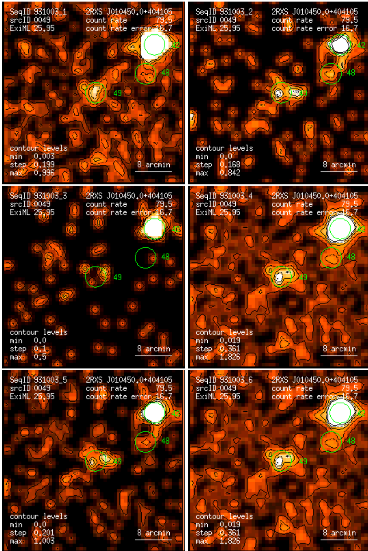
Figure 49: RASS 931003: detection 0049: band rate images, Gaussian filter: (1) PSPC channels 11 – 41, (2) 52 – 90, (3) 91 – 201, (4) 11 – 235, (5) 52 – 201, (6) 11 – 201. Broad band rates in counts/ks. Band rate contour levels in counts/ks/arcmin 2 .
