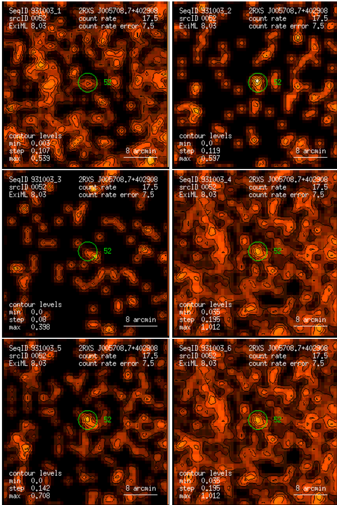
Figure 52: RASS 931003: detection 0052: band rate images, Gaussian filter: (1) PSPC channels 11 – 41, (2) 52 – 90, (3) 91 – 201, (4) 11 – 235, (5) 52 – 201, (6) 11 – 201. Broad band rates in counts/ks. Band rate contour levels in counts/ks/arcmin 2 .
