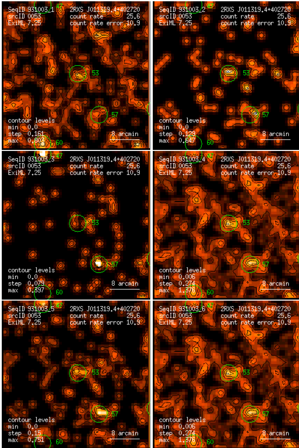
Figure 53: RASS 931003: detection 0053: band rate images, Gaussian filter: (1) PSPC channels 11 – 41, (2) 52 – 90, (3) 91 – 201, (4) 11 – 235, (5) 52 – 201, (6) 11 – 201. Broad band rates in counts/ks. Band rate contour levels in counts/ks/arcmin 2 .
