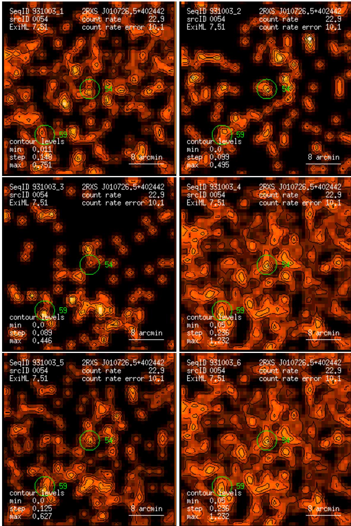
Figure 54: RASS 931003: detection 0054: band rate images, Gaussian filter: (1) PSPC channels 11 – 41, (2) 52 – 90, (3) 91 – 201, (4) 11 – 235, (5) 52 – 201, (6) 11 – 201. Broad band rates in counts/ks. Band rate contour levels in counts/ks/arcmin 2 .
