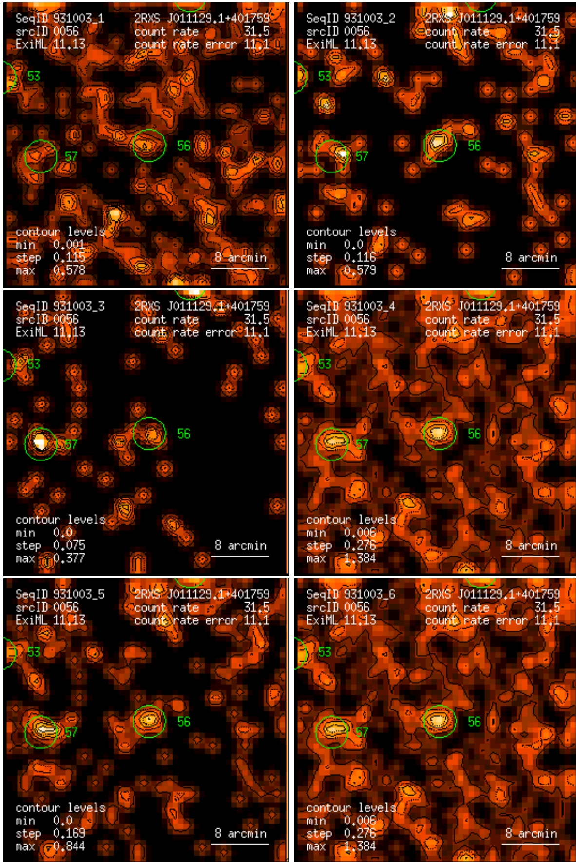
Figure 56: RASS 931003: detection 0056: band rate images, Gaussian filter: (1) PSPC channels 11 – 41, (2) 52 – 90, (3) 91 – 201, (4) 11 – 235, (5) 52 – 201, (6) 11 – 201. Broad band rates in counts/ks. Band rate contour levels in counts/ks/arcmin 2 .
