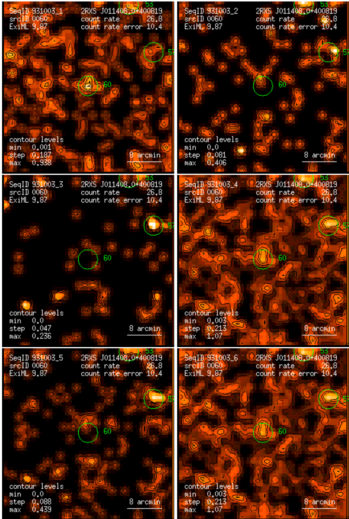
Figure 60: RASS 931003: detection 0060: band rate images, Gaussian filter: (1) PSPC channels 11 – 41, (2) 52 – 90, (3) 91 – 201, (4) 11 – 235, (5) 52 – 201, (6) 11 – 201. Broad band rates in counts/ks. Band rate contour levels in counts/ks/arcmin 2 .
