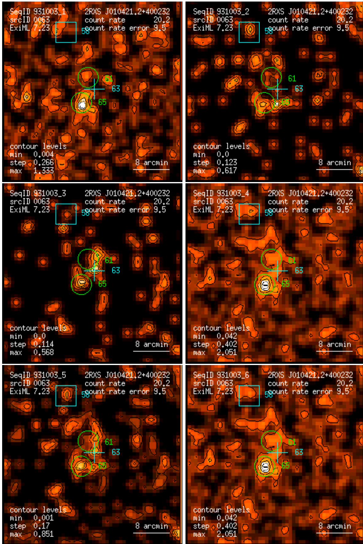
Figure 63: RASS 931003: detection 0063: band rate images, Gaussian filter: (1) PSPC channels 11 – 41, (2) 52 – 90, (3) 91 – 201, (4) 11 – 235, (5) 52 – 201, (6) 11 – 201. Broad band rates in counts/ks. Band rate contour levels in counts/ks/arcmin 2 .
