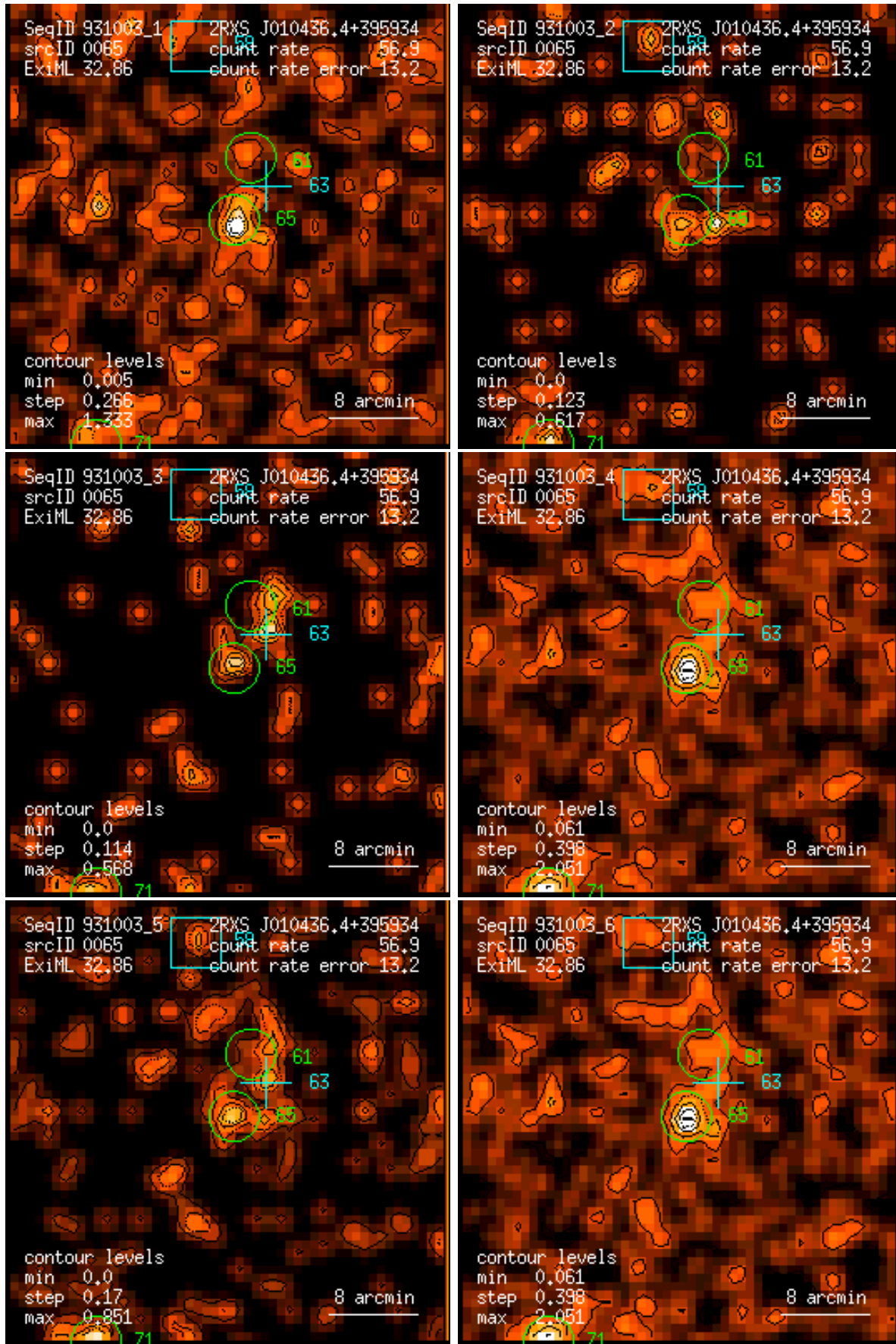
Figure 65: RASS 931003: detection 0065: band rate images, Gaussian filter: (1) PSPC channels 11 – 41, (2) 52 – 90, (3) 91 – 201, (4) 11 – 235, (5) 52 – 201, (6) 11 – 201. Broad band rates in counts/ks. Band rate contour levels in counts/ks/arcmin 2 .
