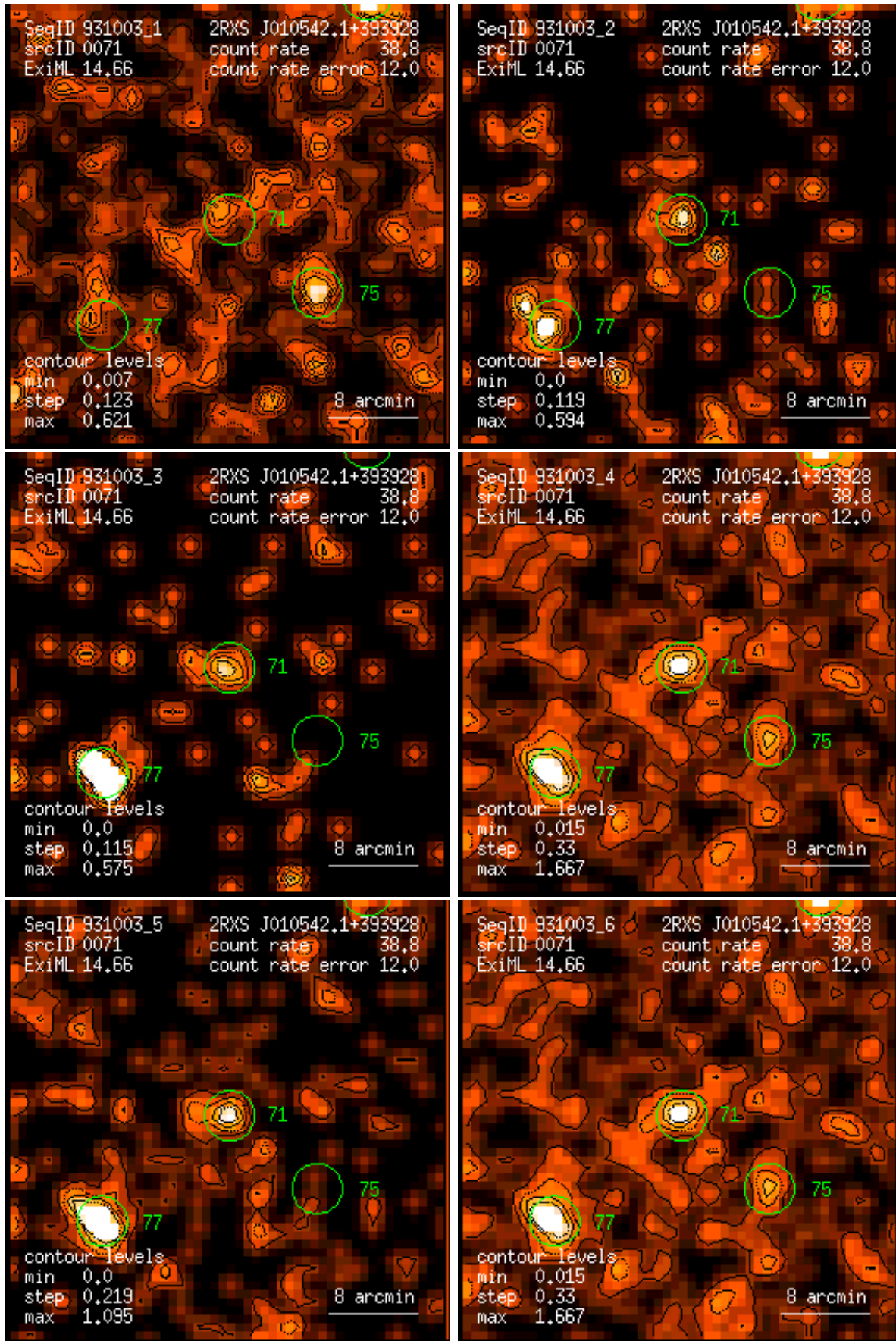
Figure 71: RASS 931003: detection 0071: band rate images, Gaussian filter: (1) PSPC channels 11 – 41, (2) 52 – 90, (3) 91 – 201, (4) 11 – 235, (5) 52 – 201, (6) 11 – 201. Broad band rates in counts/ks. Band rate contour levels in counts/ks/arcmin 2 .
