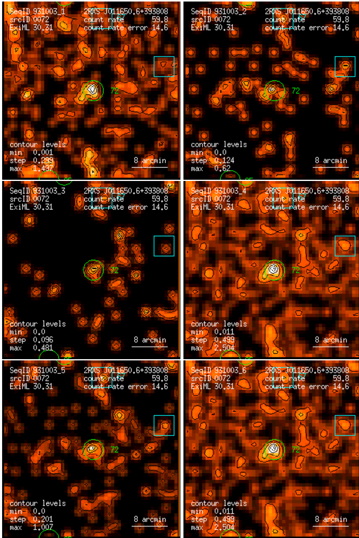
Figure 72: RASS 931003: detection 0072: band rate images, Gaussian filter: (1) PSPC channels 11 – 41, (2) 52 – 90, (3) 91 – 201, (4) 11 – 235, (5) 52 – 201, (6) 11 – 201. Broad band rates in counts/ks. Band rate contour levels in counts/ks/arcmin 2 .
