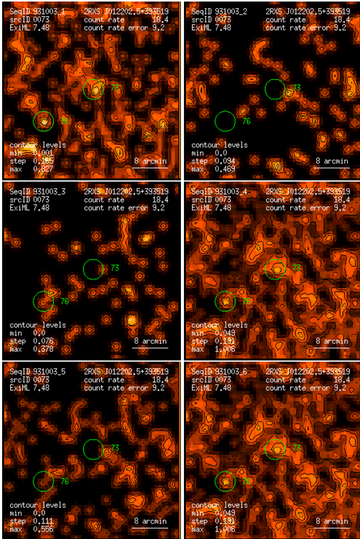
Figure 73: RASS 931003: detection 0073: band rate images, Gaussian filter: (1) PSPC channels 11 – 41, (2) 52 – 90, (3) 91 – 201, (4) 11 – 235, (5) 52 – 201, (6) 11 – 201. Broad band rates in counts/ks. Band rate contour levels in counts/ks/arcmin 2 .
